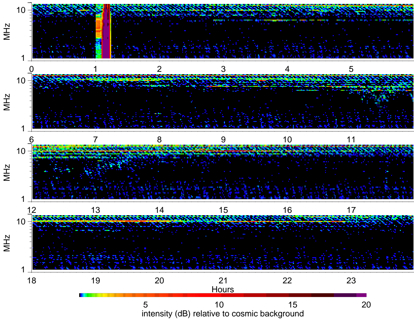
Wind Waves RAD2 receiver: 1996/8/7
