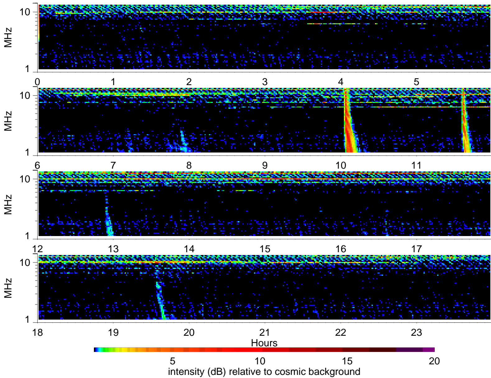
Wind Waves RAD2 receiver: 1996/8/4
