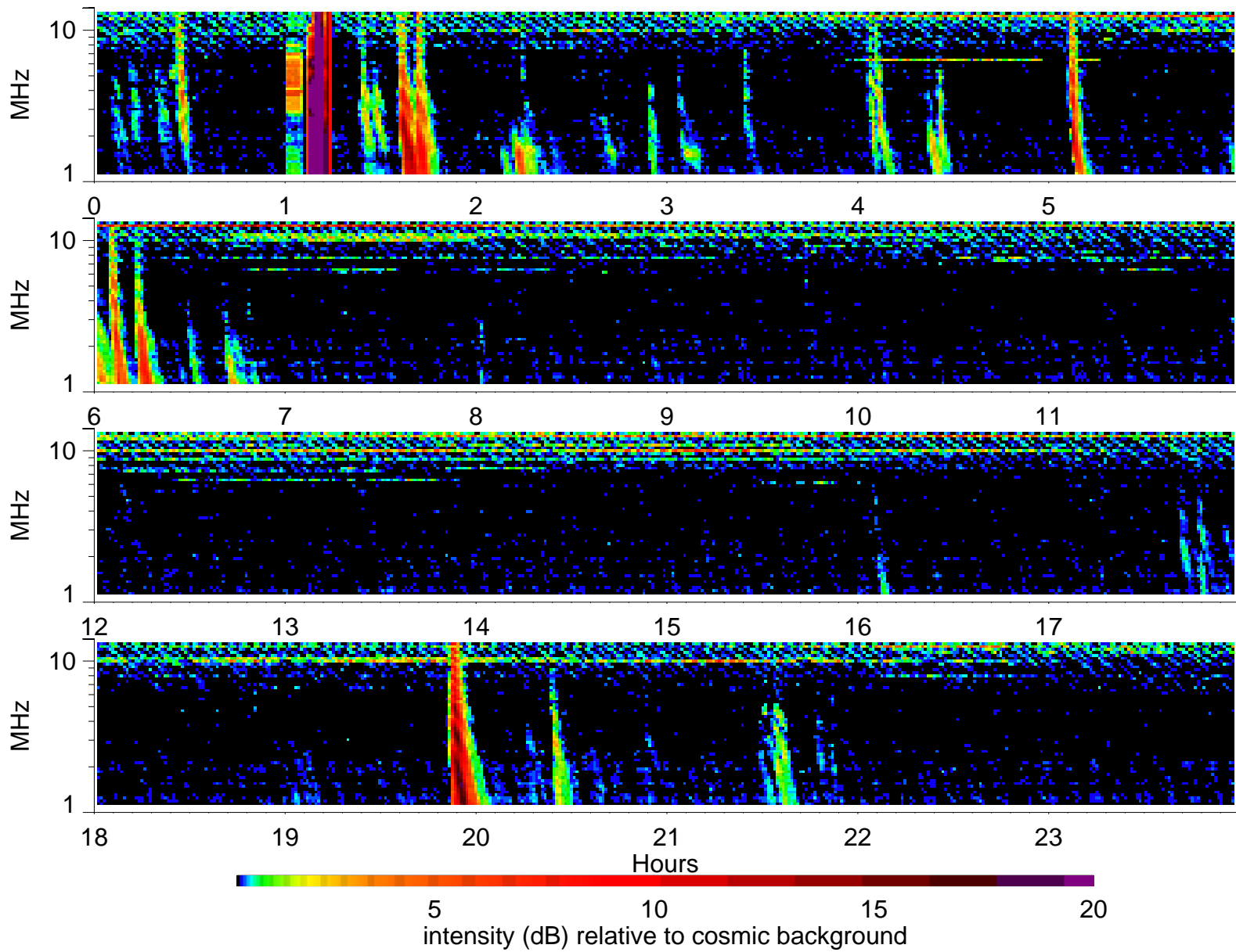
Wind Waves RAD2 receiver: 1996/8/3
