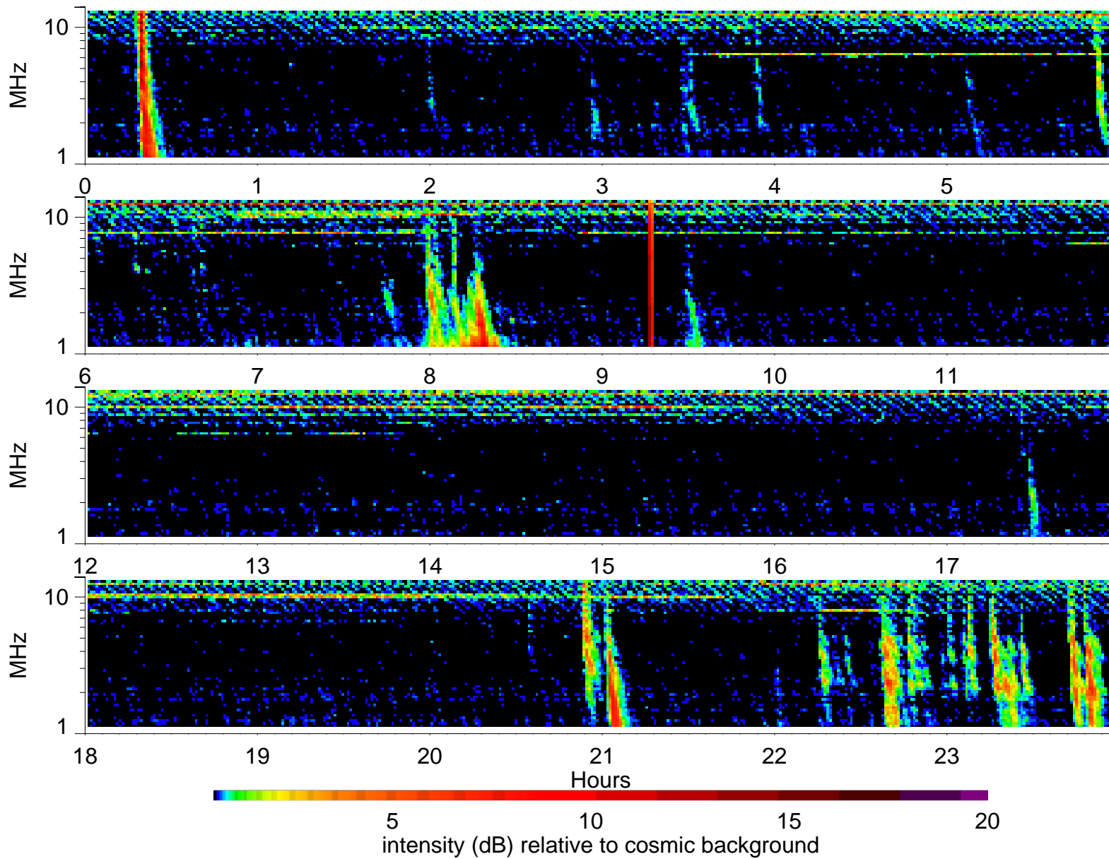
Wind Waves RAD2 receiver: 1996/8/2
