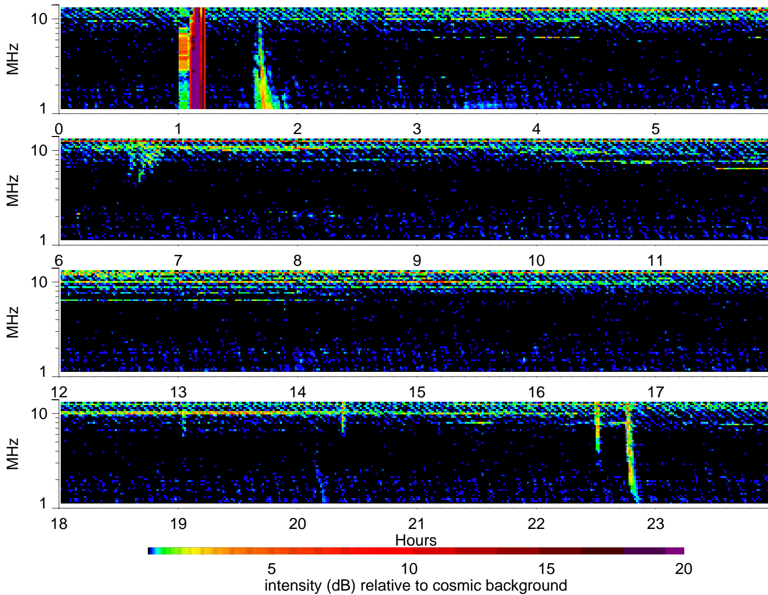
Wind Waves RAD2 receiver: 1996/8/1
