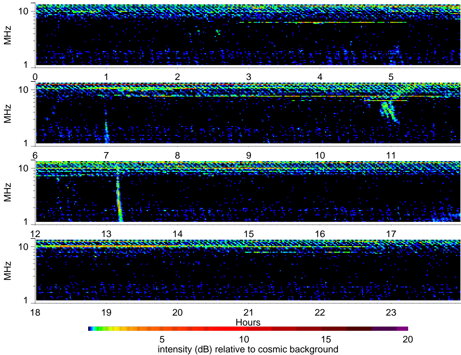
Wind Waves RAD2 receiver: 1996/7/31
