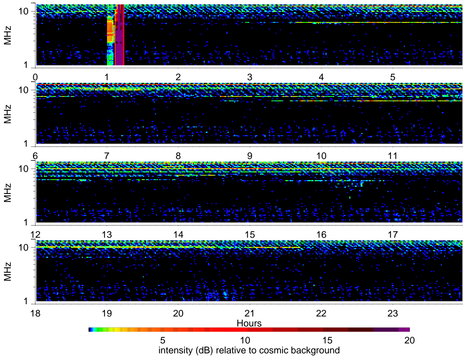
Wind Waves RAD2 receiver: 1996/7/28
