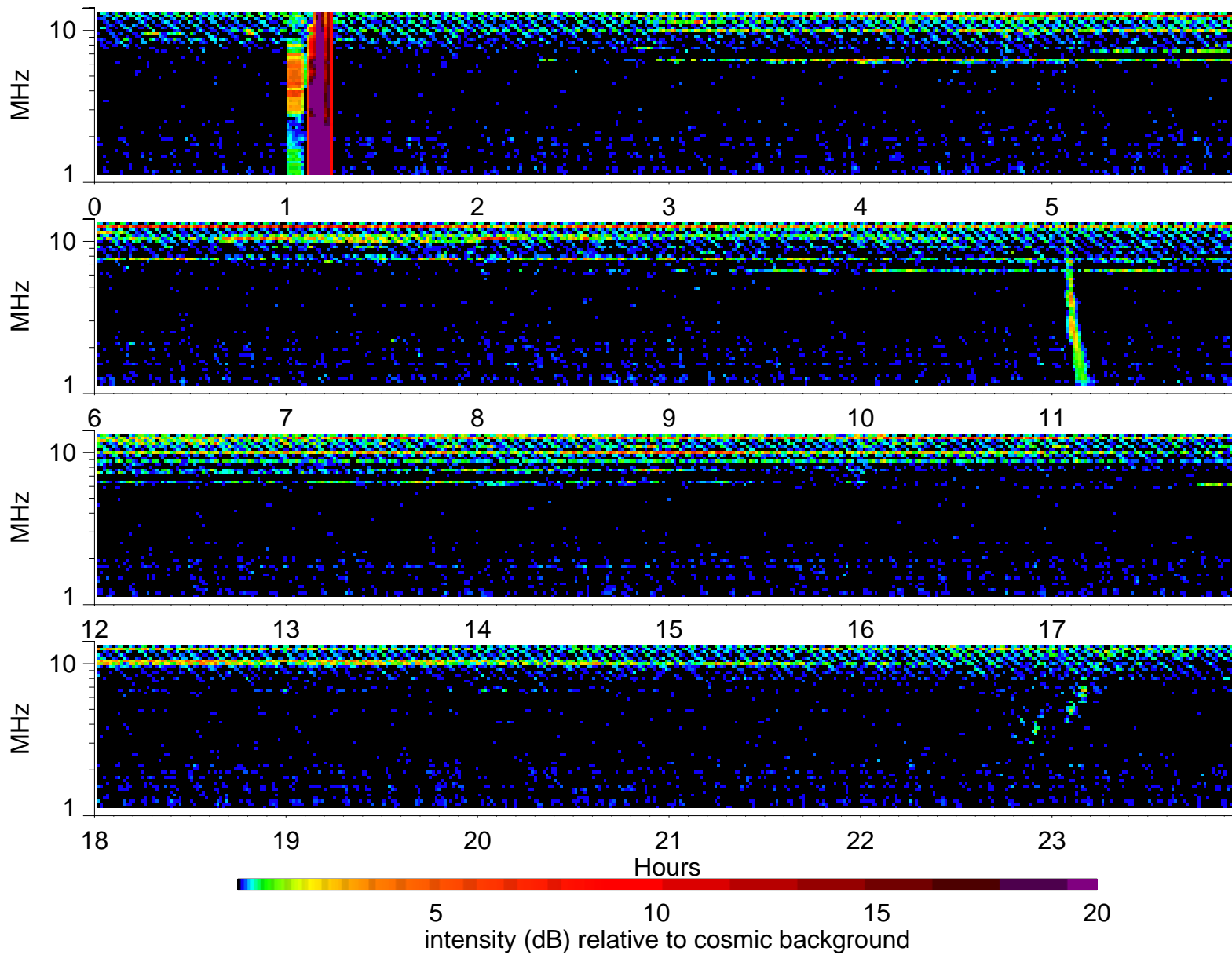
Wind Waves RAD2 receiver: 1996/7/26
