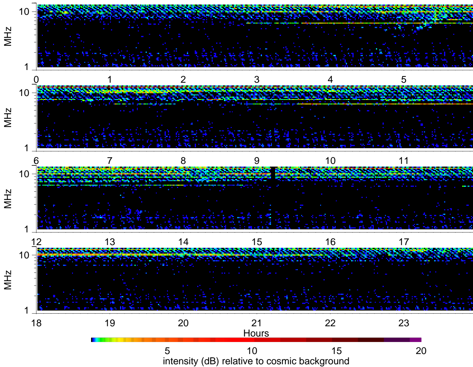
Wind Waves RAD2 receiver: 1996/7/25
