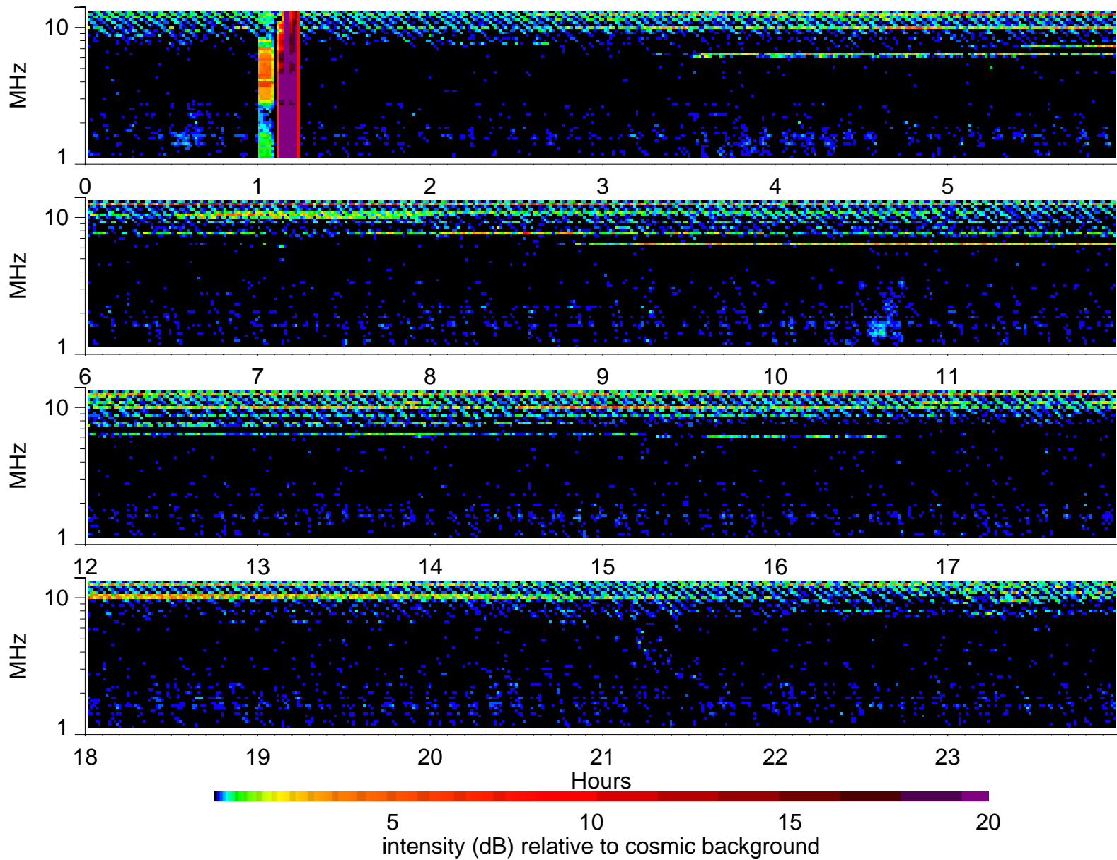
Wind Waves RAD2 receiver: 1996/7/20
