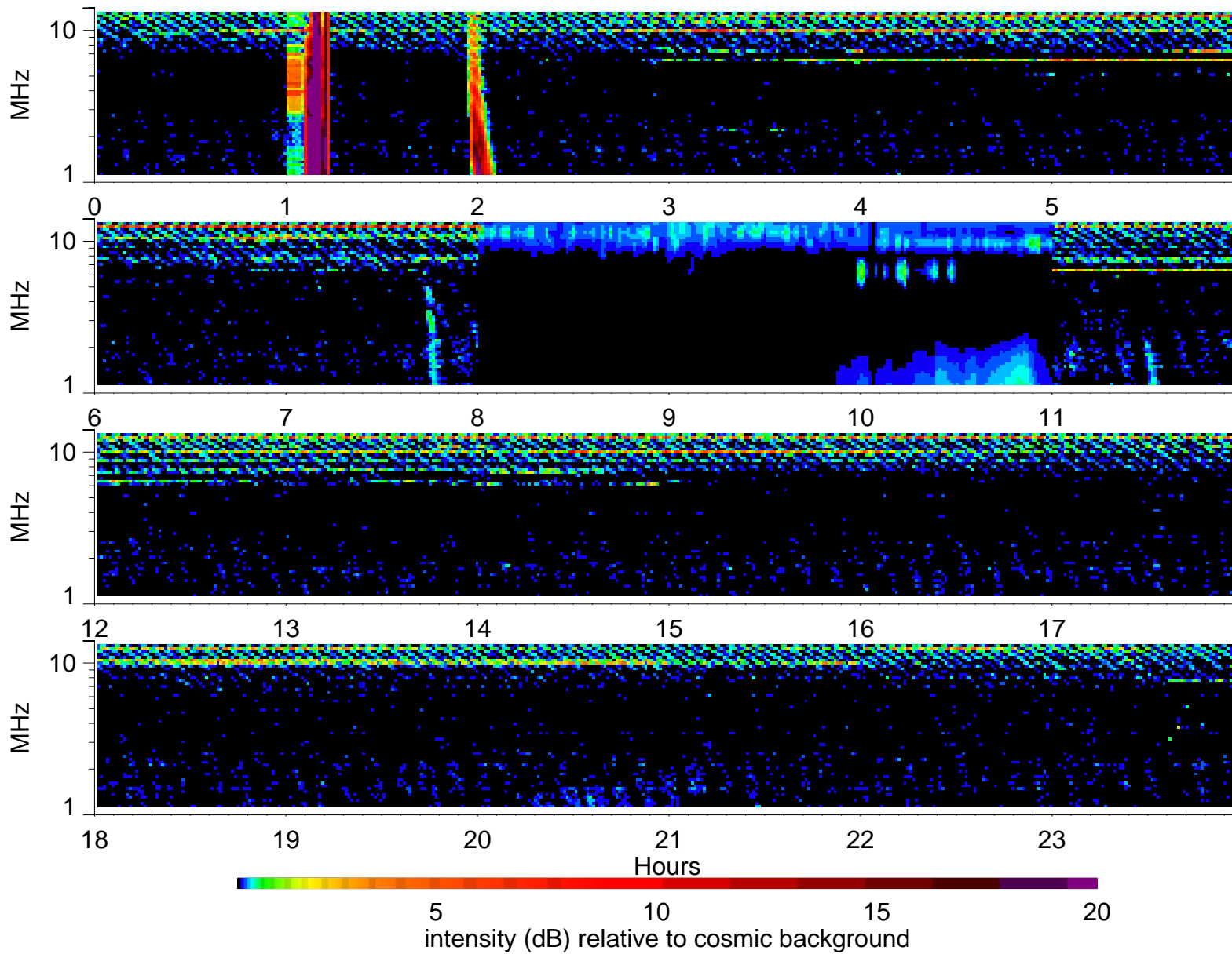
Wind Waves RAD2 receiver: 1996/7/16
