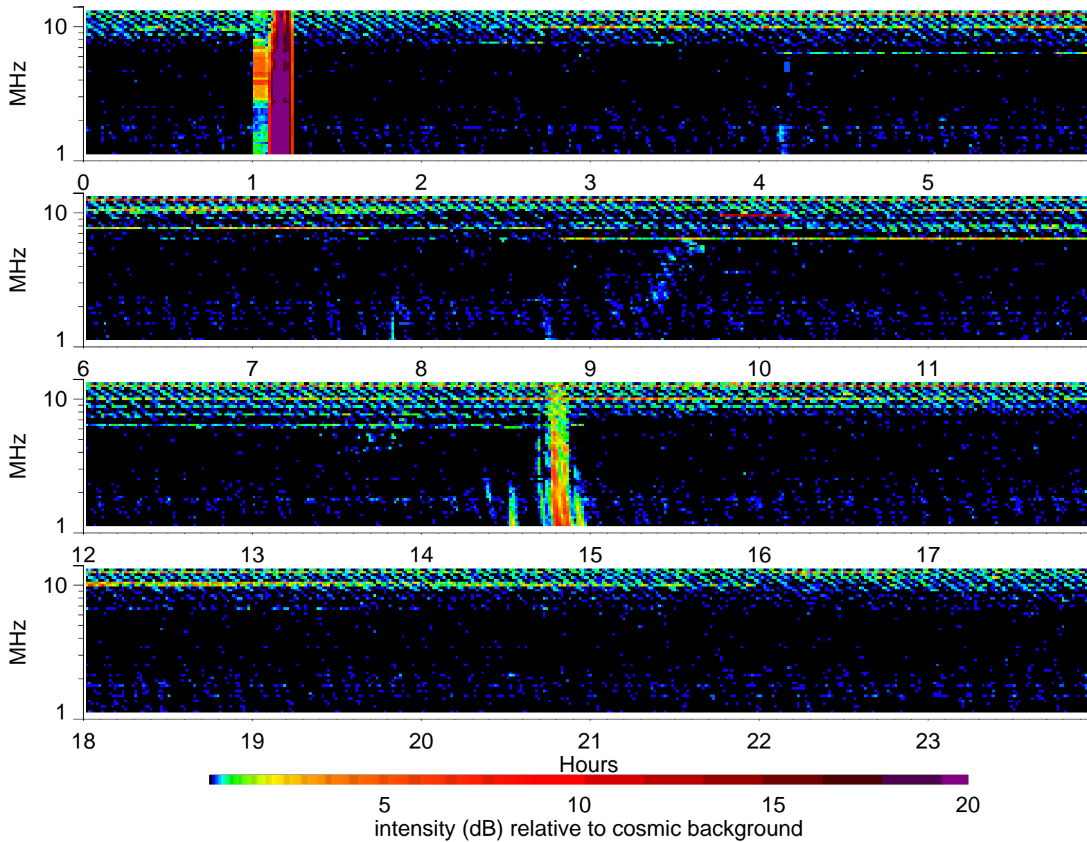
Wind Waves RAD2 receiver: 1996/7/14
