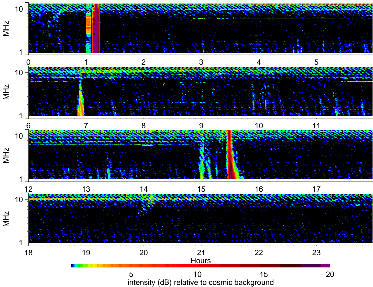
Wind Waves RAD2 receiver: 1996/7/12
