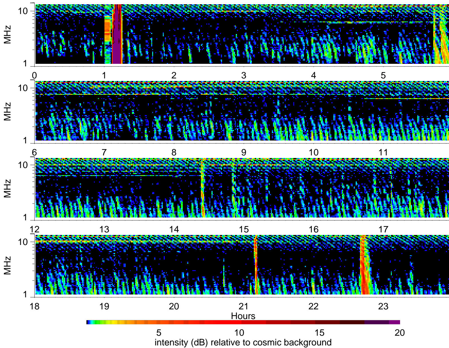
Wind Waves RAD2 receiver: 1996/7/10
