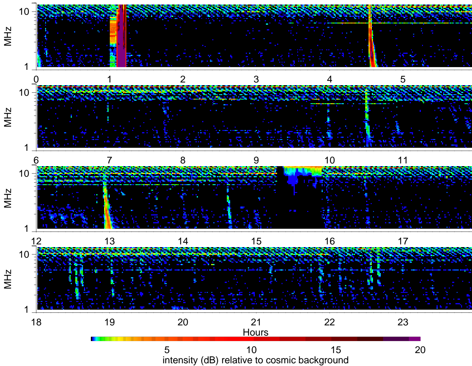
Wind Waves RAD2 receiver: 1996/7/8
