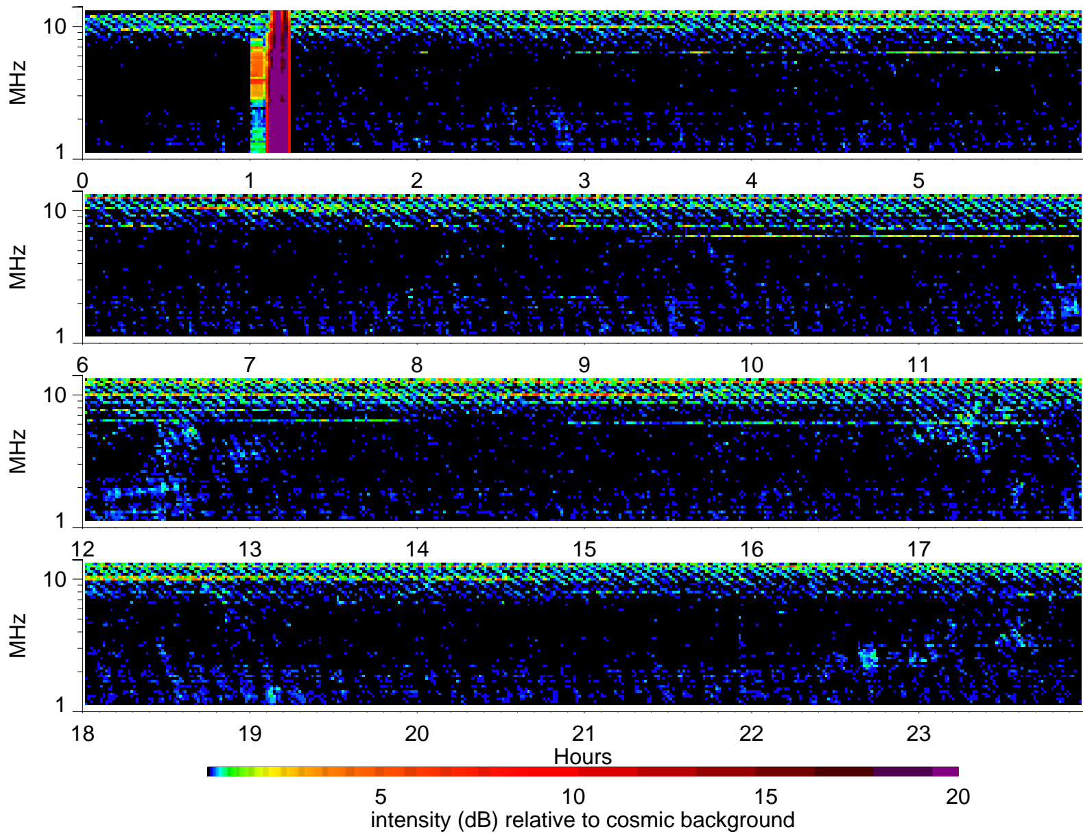
Wind Waves RAD2 receiver: 1996/7/6
