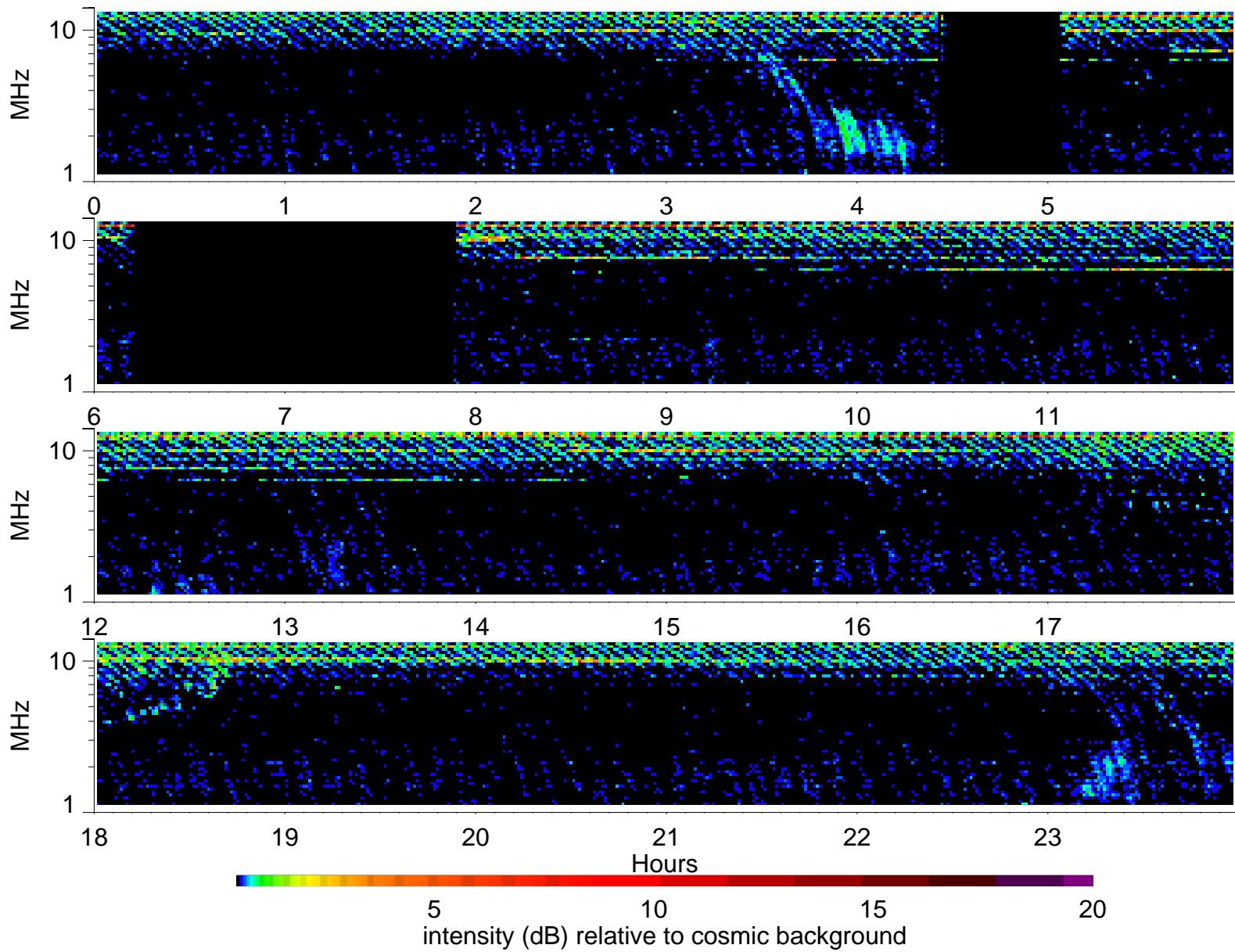
Wind Waves RAD2 receiver: 1996/7/5
