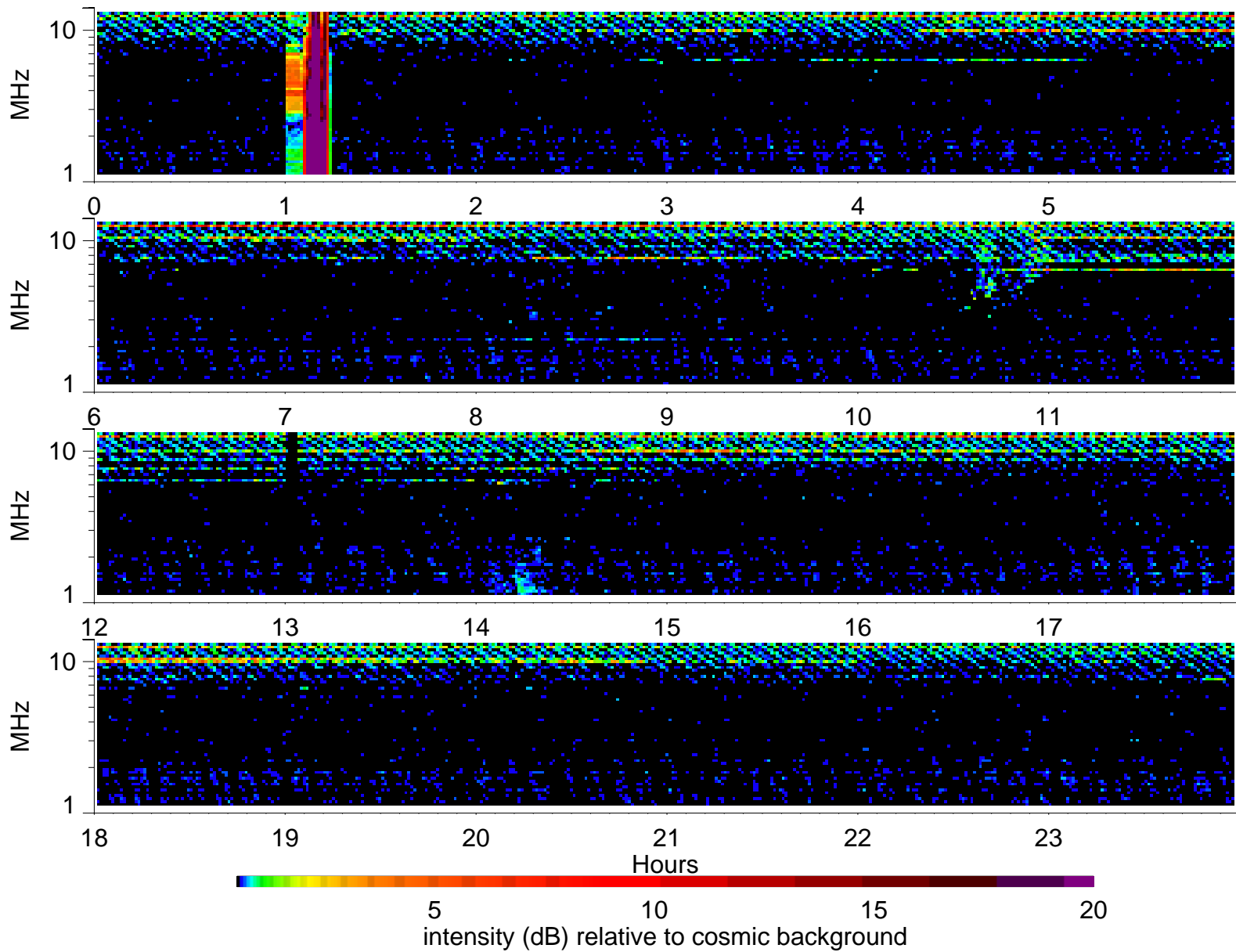
Wind Waves RAD2 receiver: 1996/6/30
