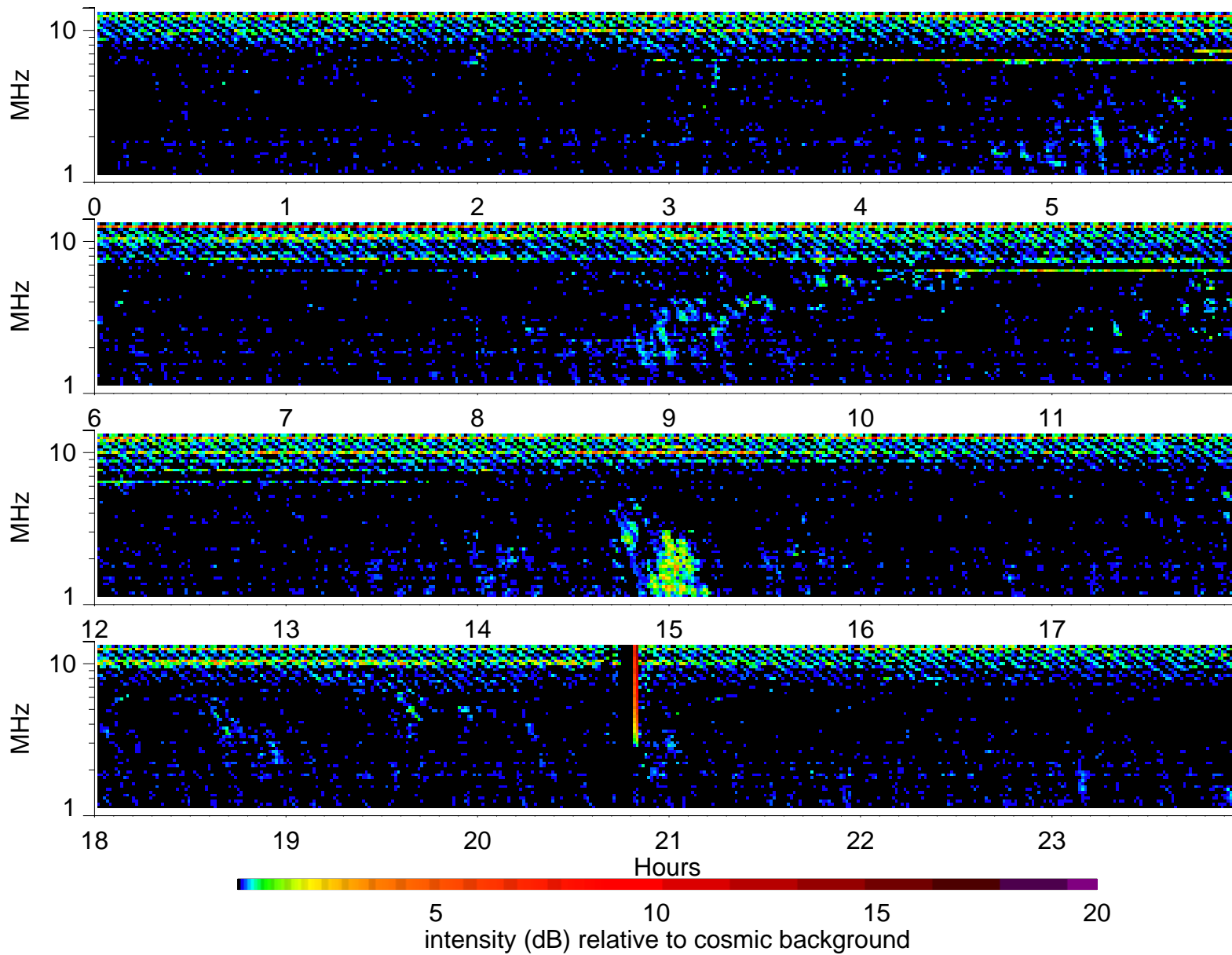
Wind Waves RAD2 receiver: 1996/6/25
