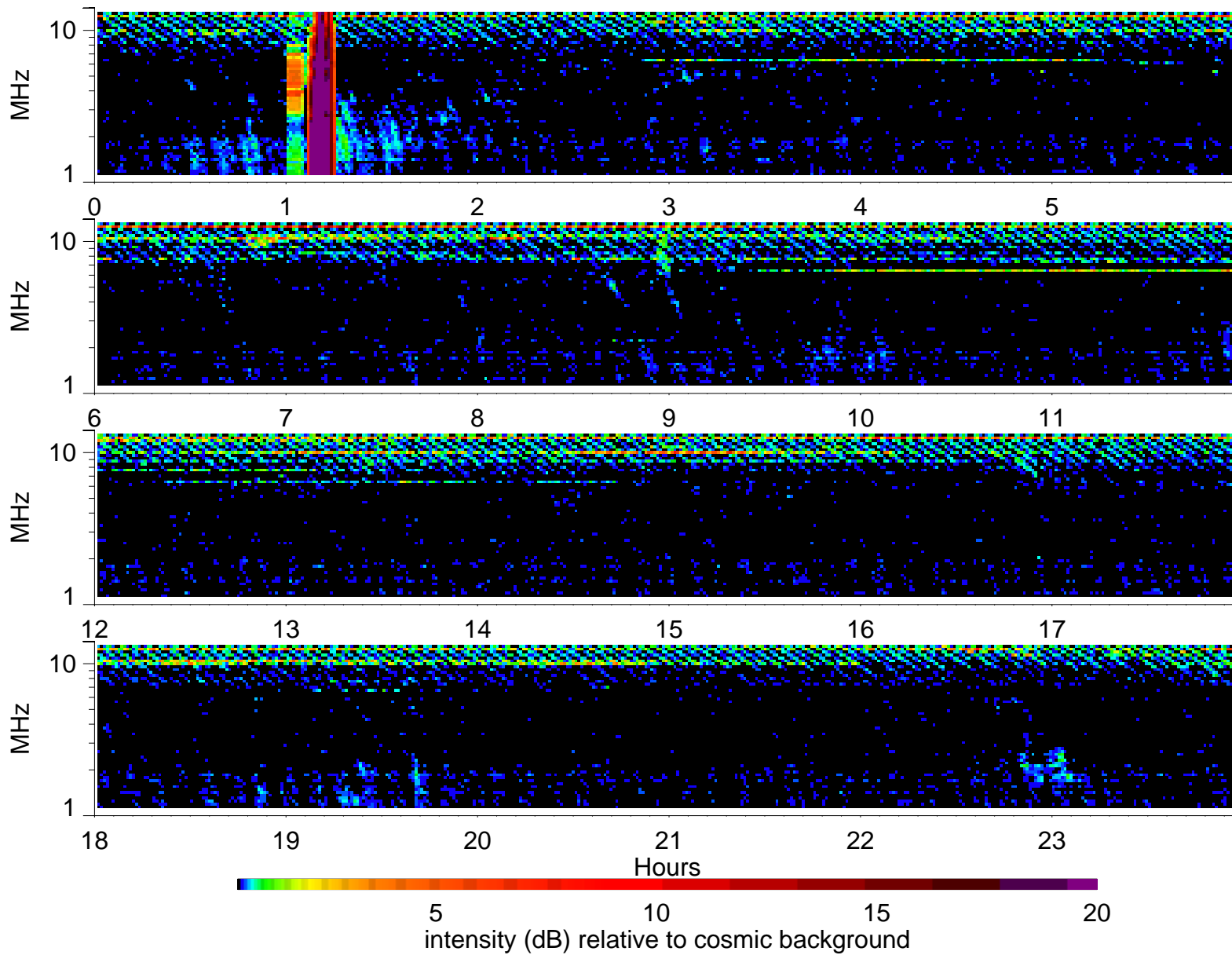
Wind Waves RAD2 receiver: 1996/6/24
