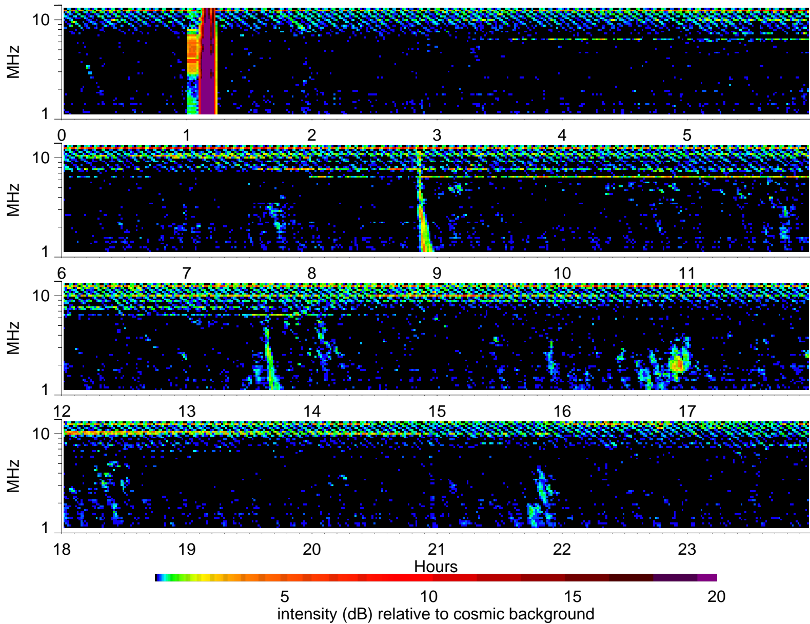
Wind Waves RAD2 receiver: 1996/6/22
