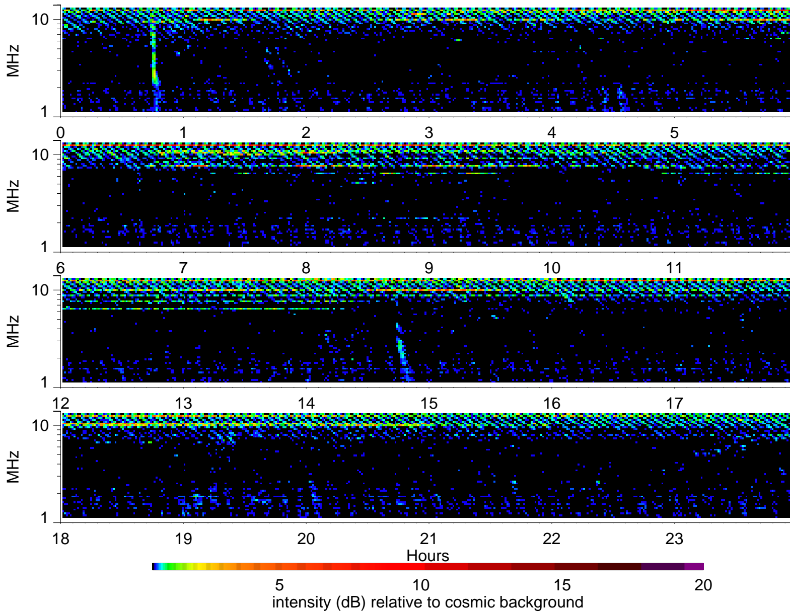
Wind Waves RAD2 receiver: 1996/6/19
