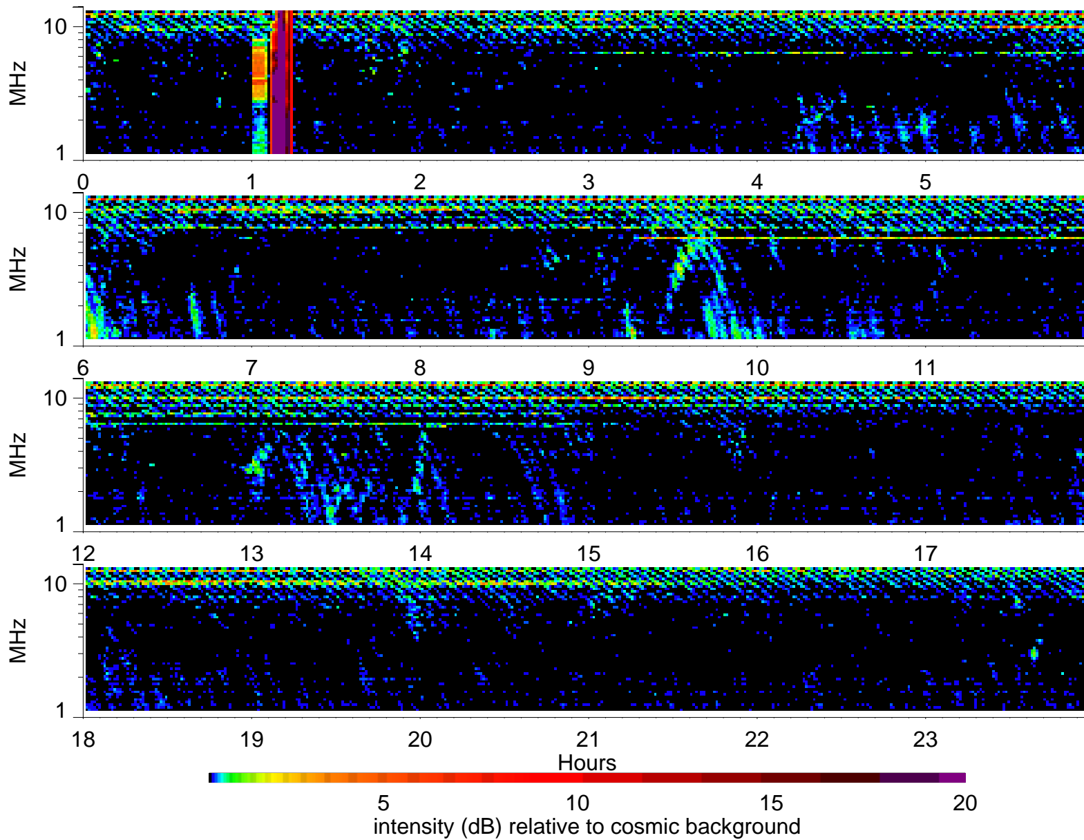
Wind Waves RAD2 receiver: 1996/6/18
