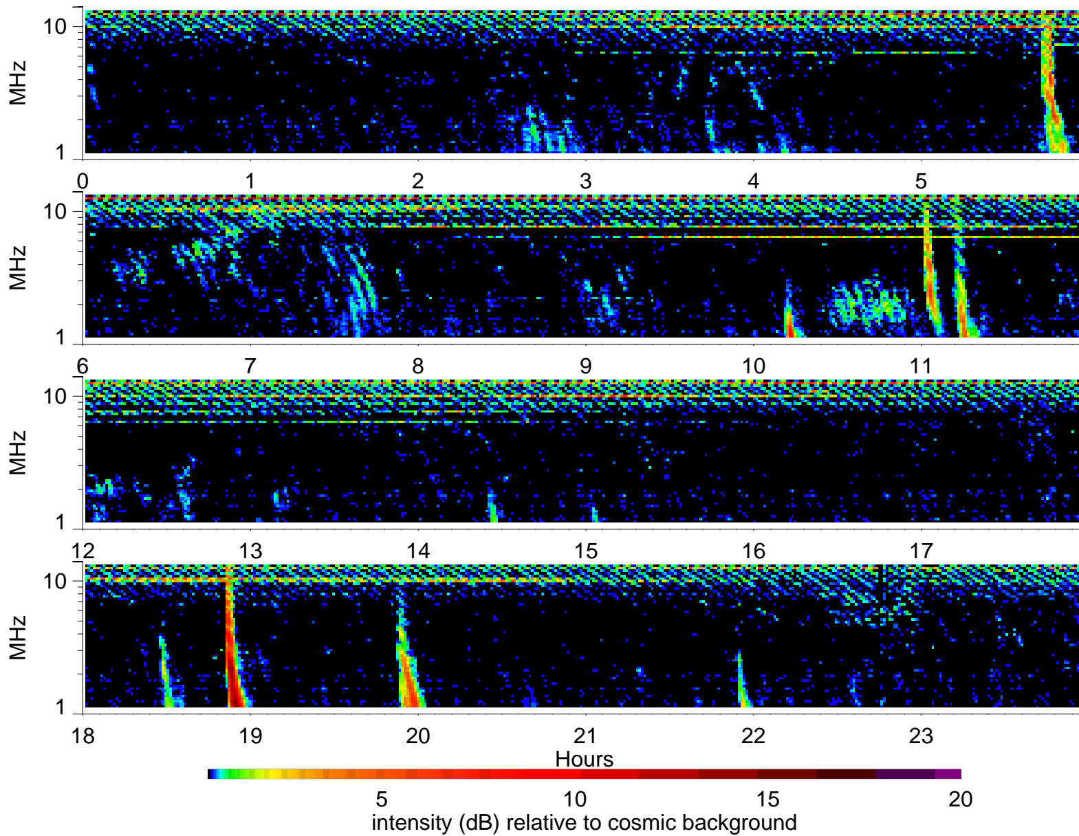
Wind Waves RAD2 receiver: 1996/6/17
