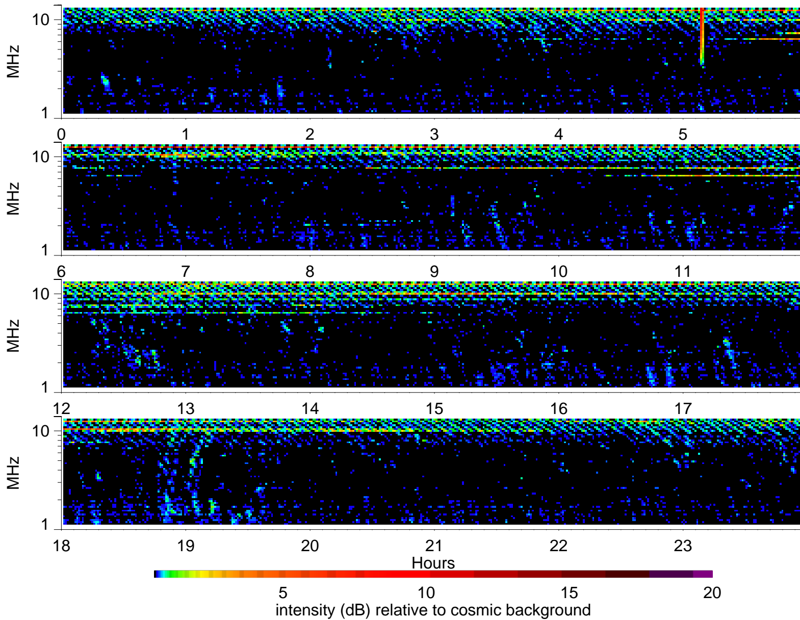
Wind Waves RAD2 receiver: 1996/6/15
