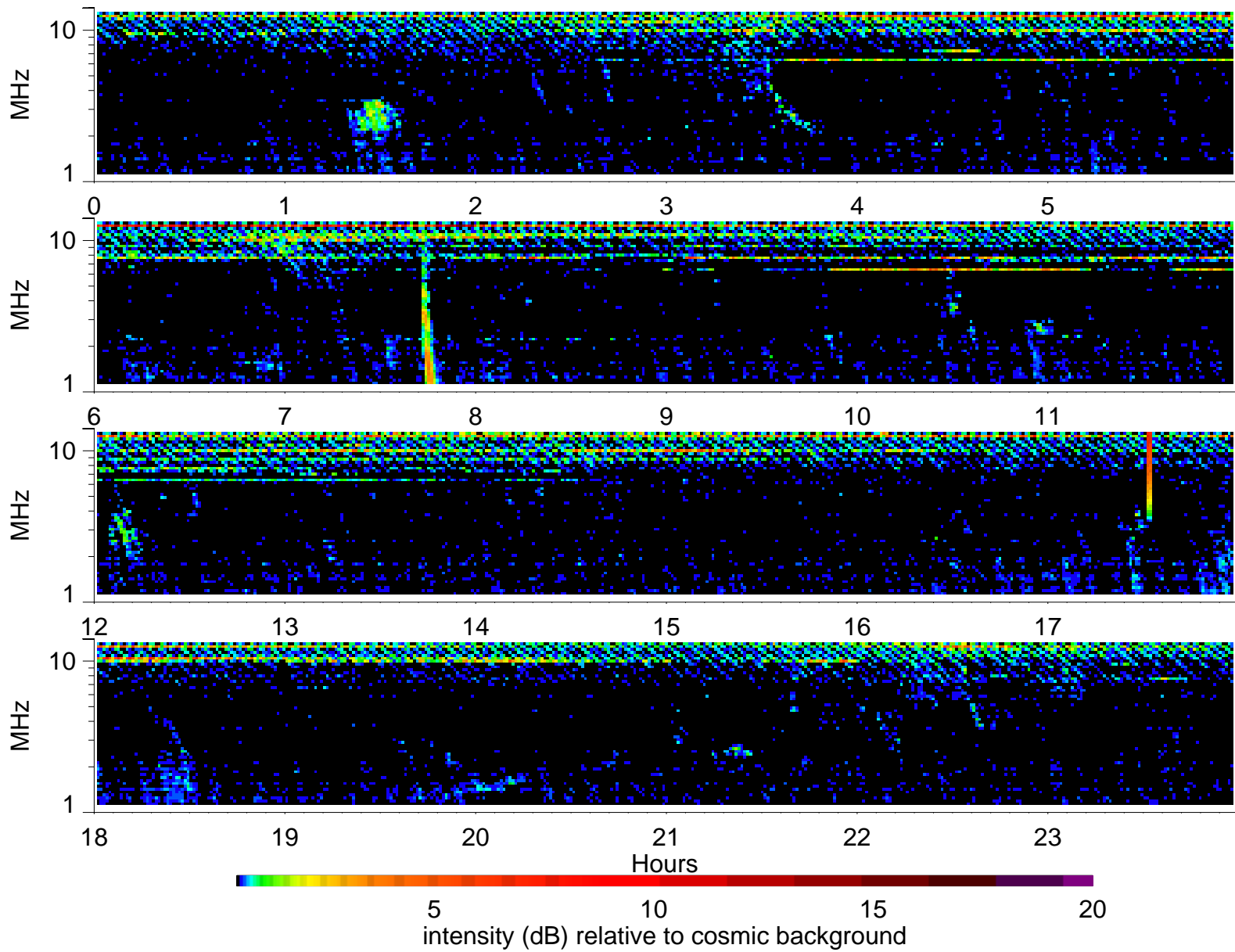
Wind Waves RAD2 receiver: 1996/6/3
