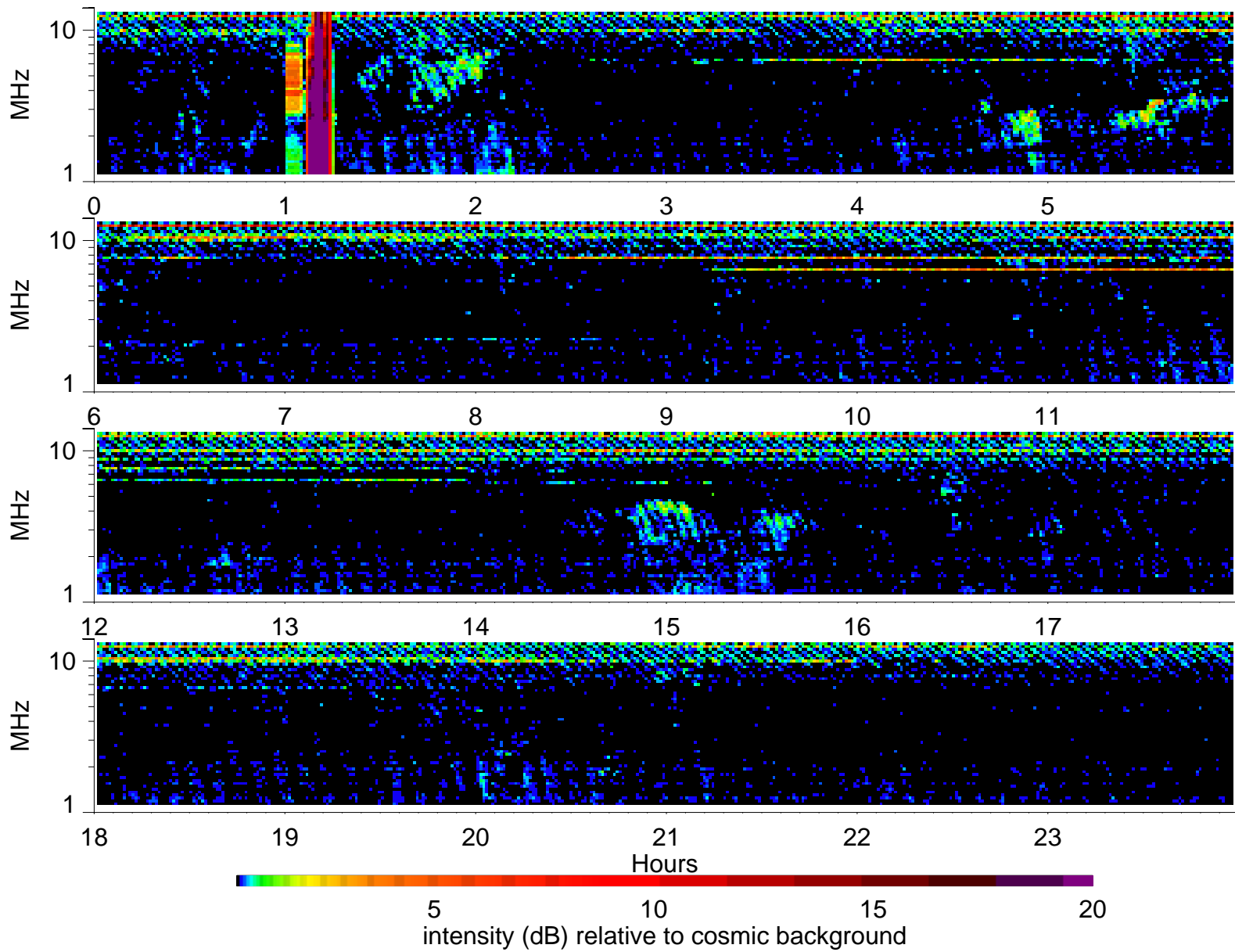
Wind Waves RAD2 receiver: 1996/6/2
