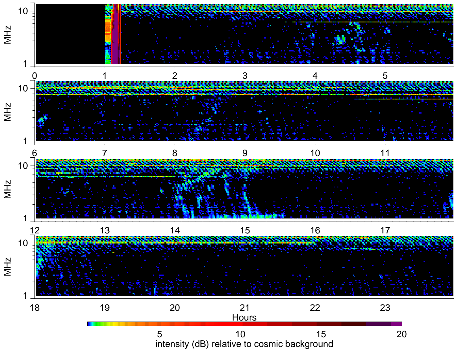
Wind Waves RAD2 receiver: 1996/5/31
