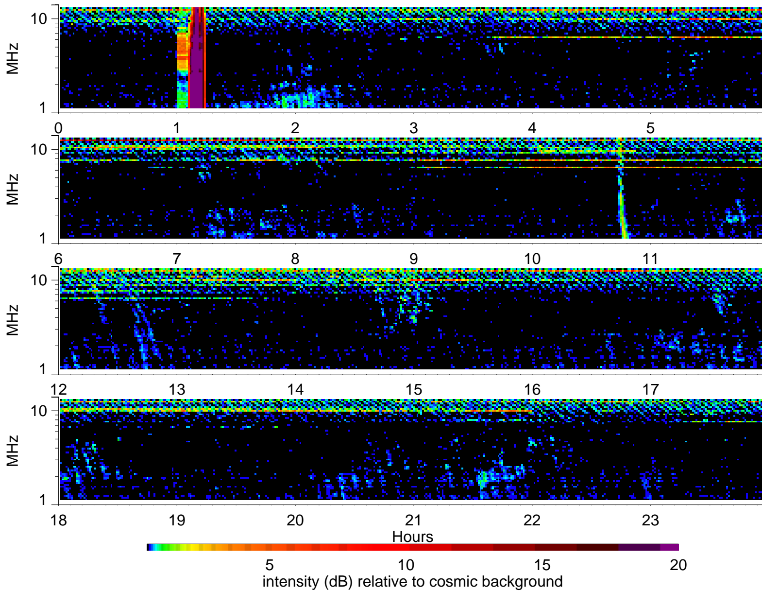
Wind Waves RAD2 receiver: 1996/5/29
