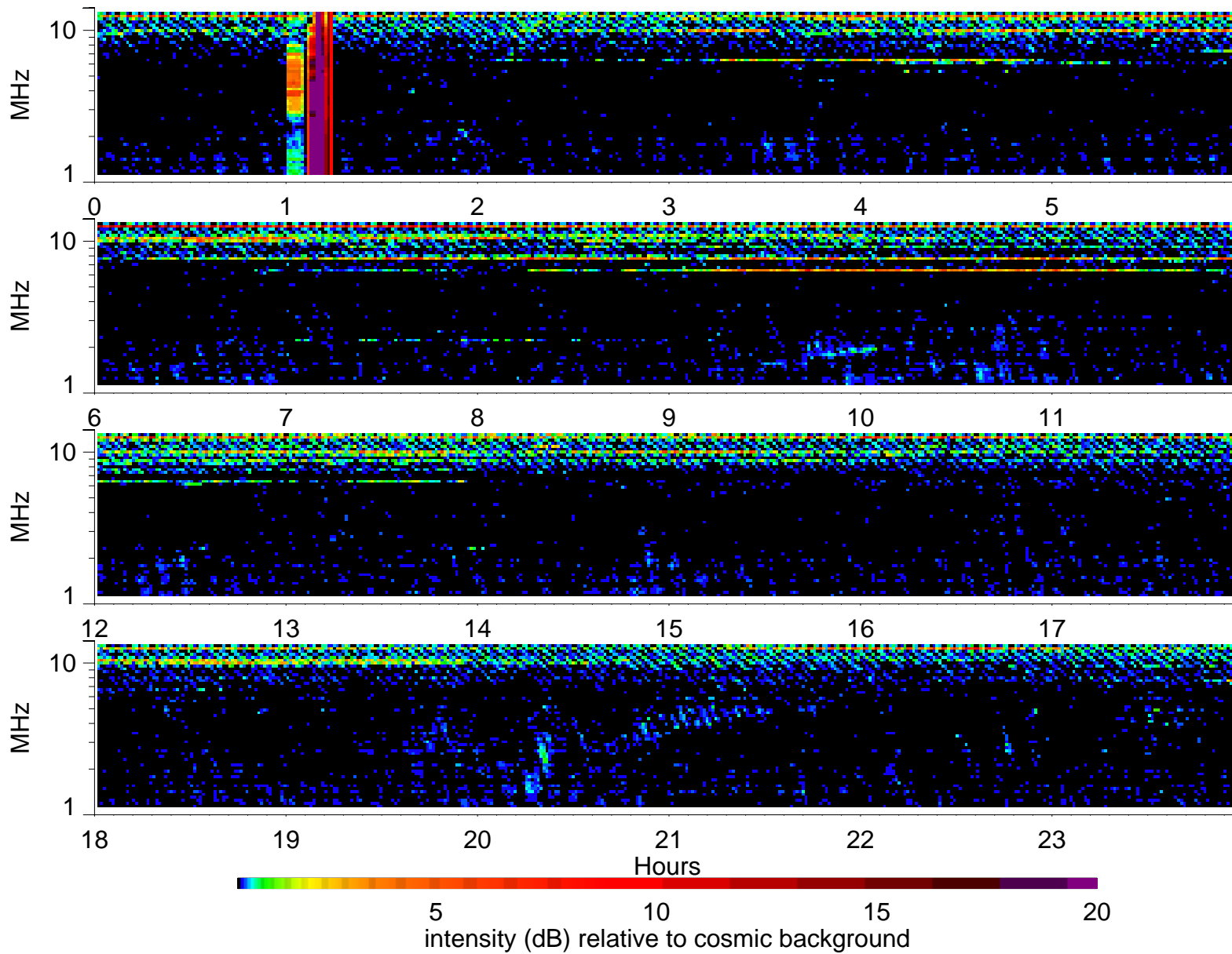
Wind Waves RAD2 receiver: 1996/5/27
