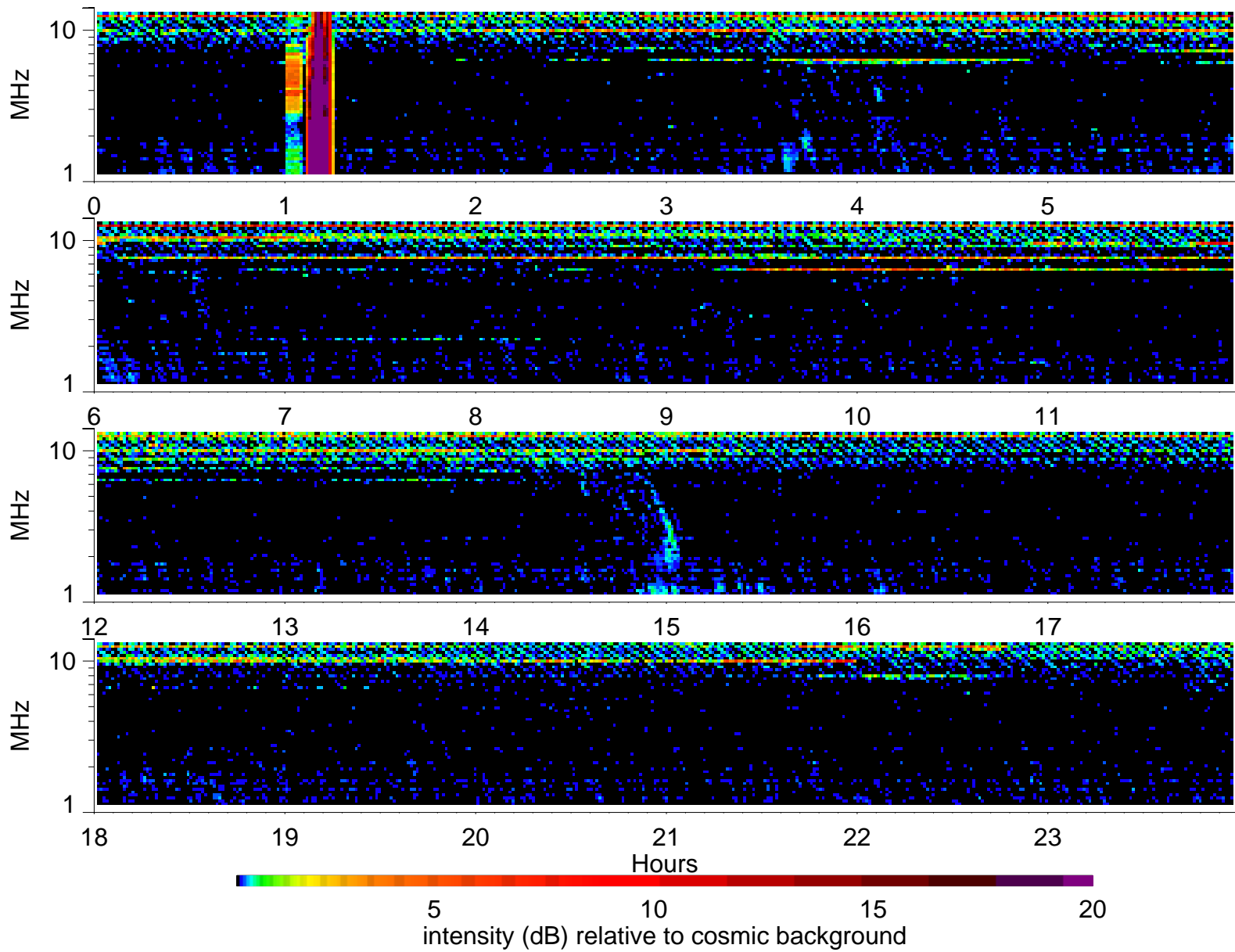
Wind Waves RAD2 receiver: 1996/5/25
