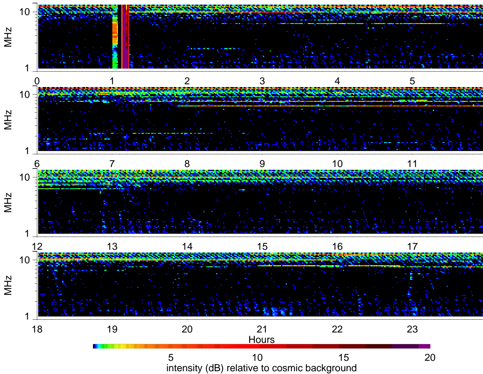
Wind Waves RAD2 receiver: 1996/5/23
