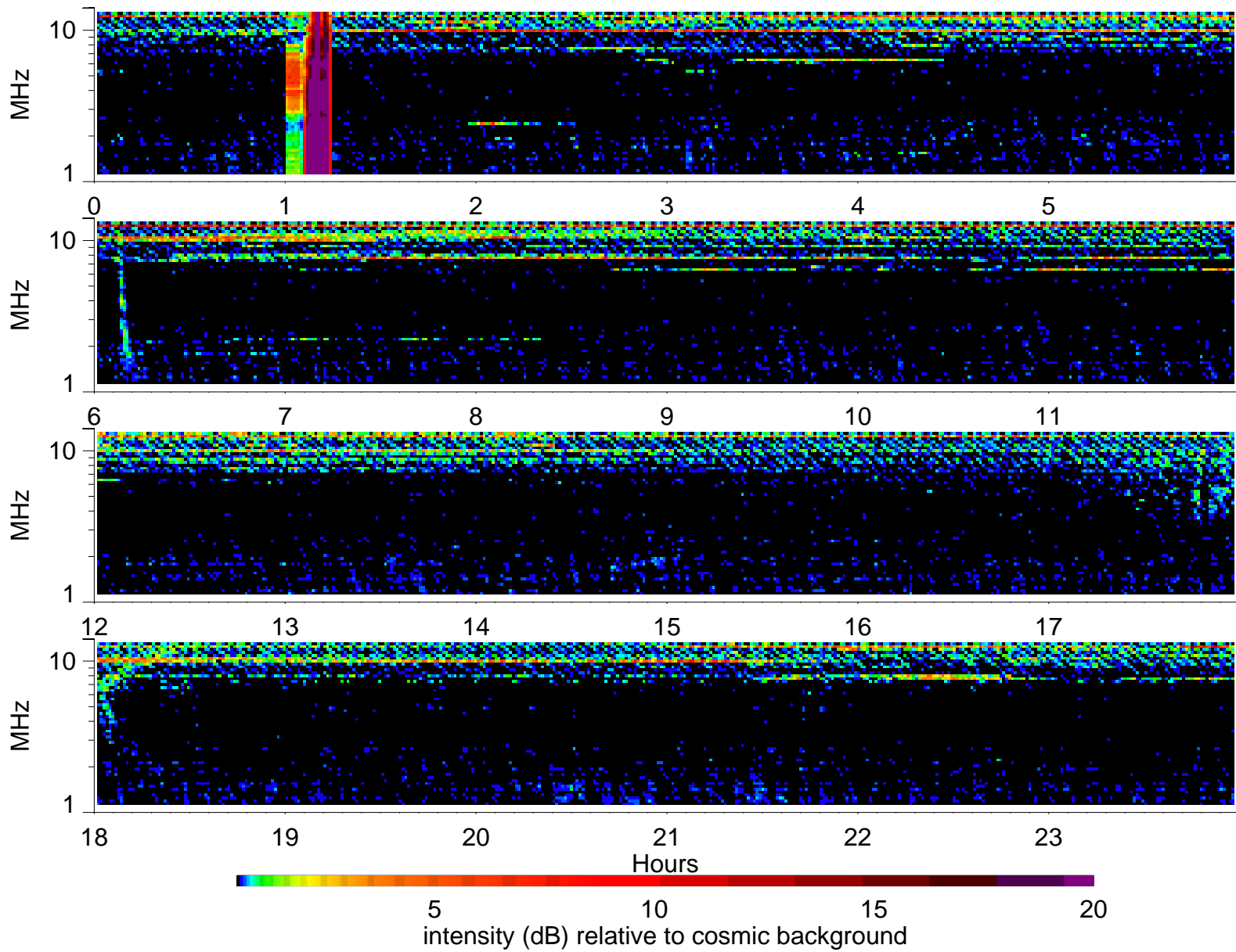
Wind Waves RAD2 receiver: 1996/5/21
