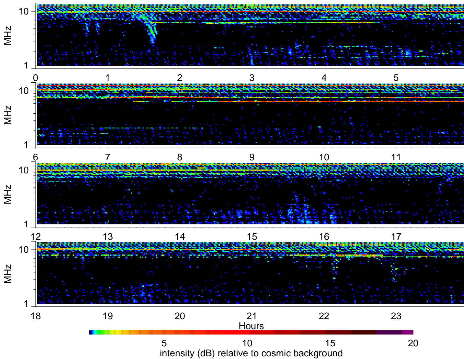
Wind Waves RAD2 receiver: 1996/5/20
