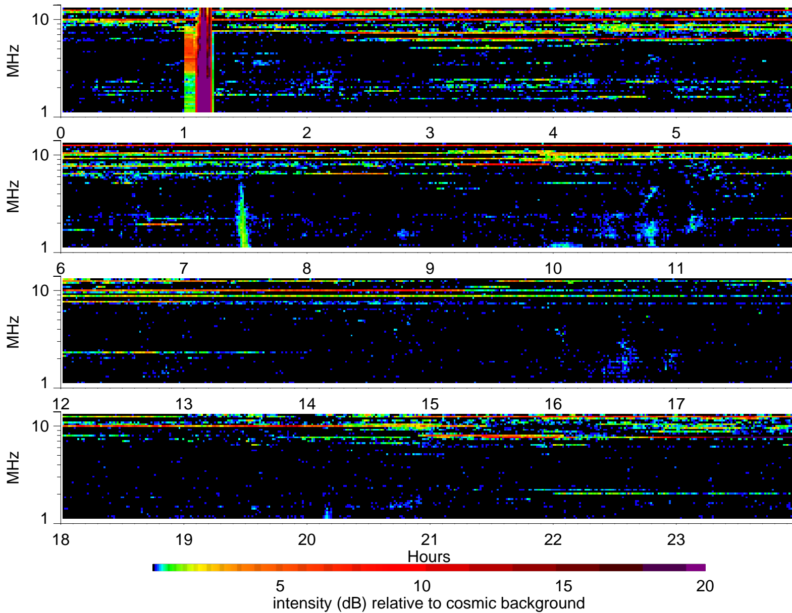
Wind Waves RAD2 receiver: 1996/5/15
