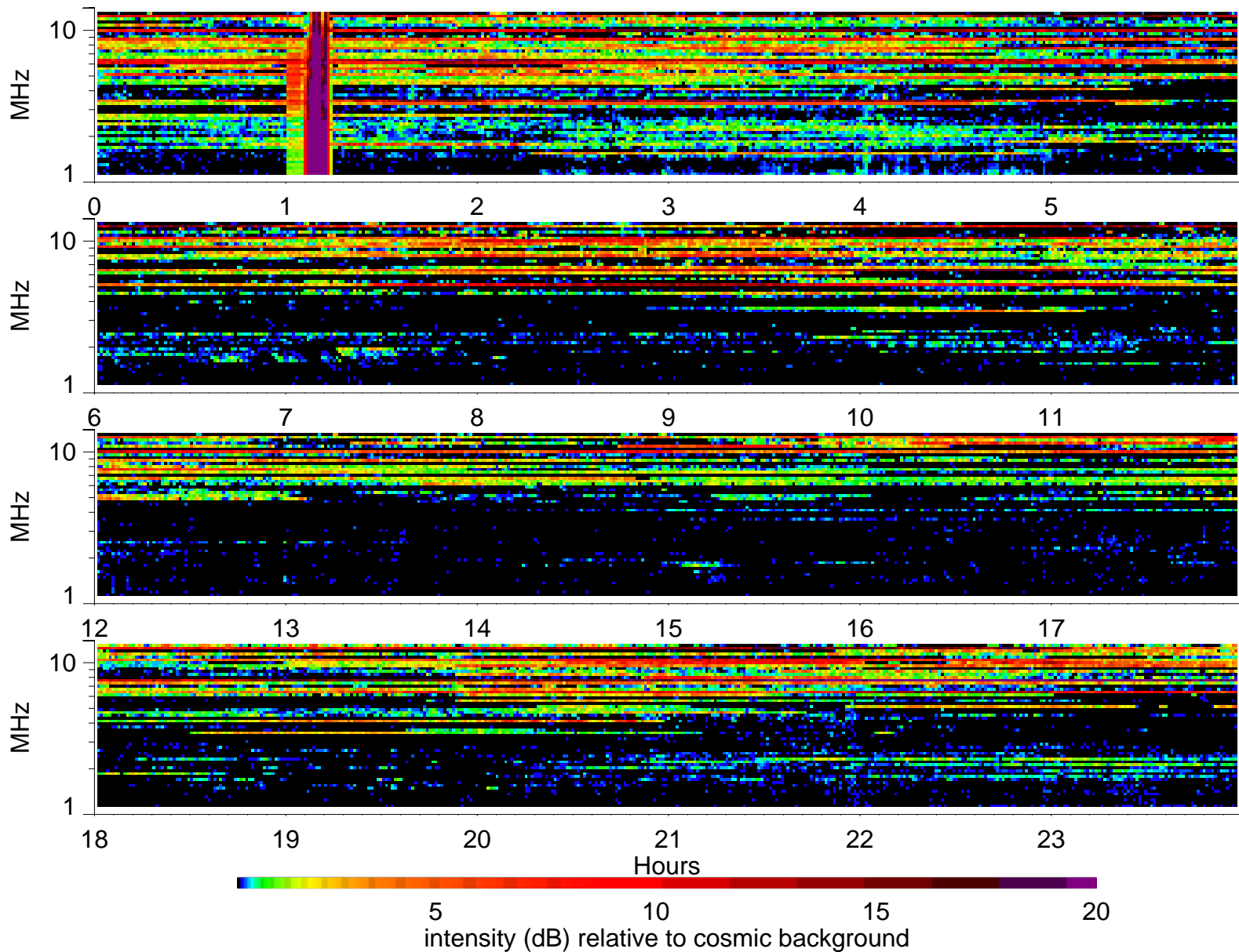
Wind Waves RAD2 receiver: 1996/5/11
