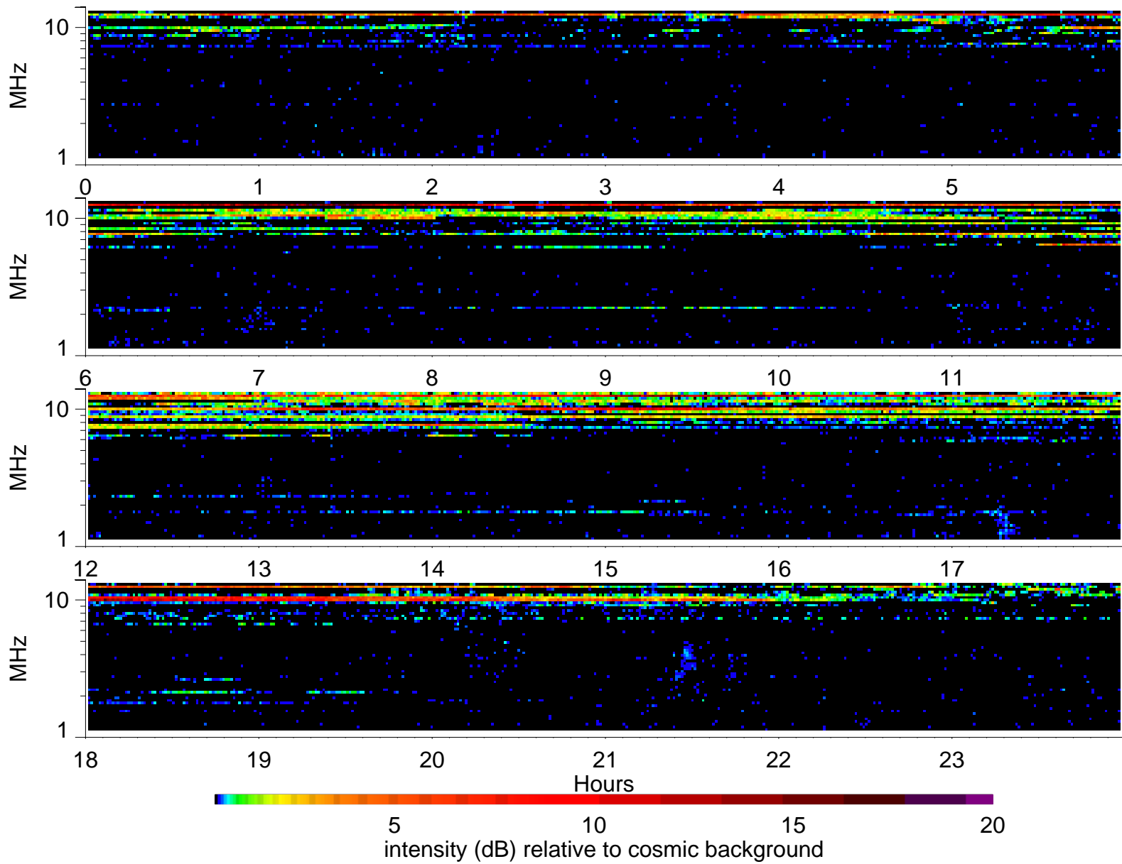
Wind Waves RAD2 receiver: 1996/5/4
