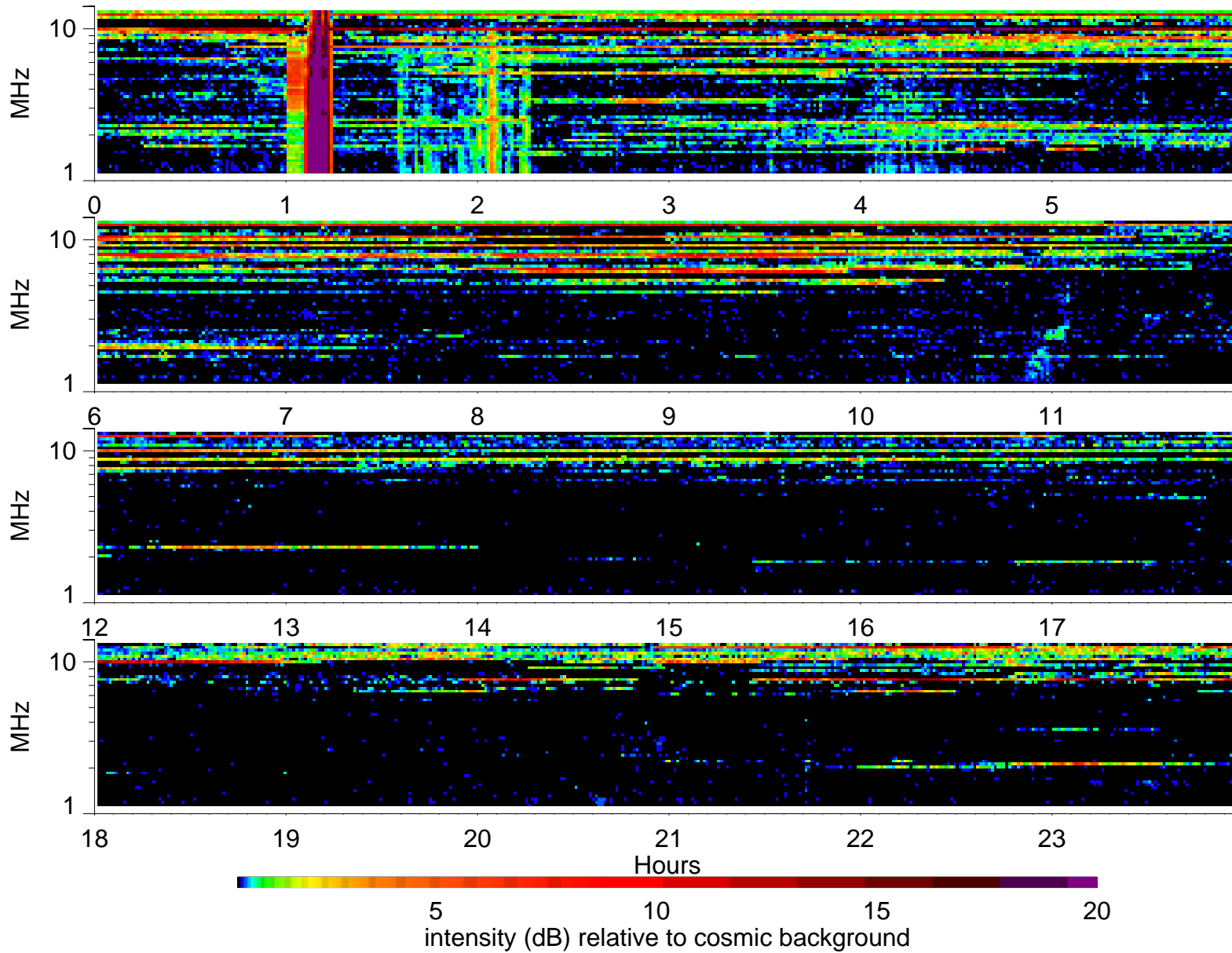
Wind Waves RAD2 receiver: 1996/4/21
