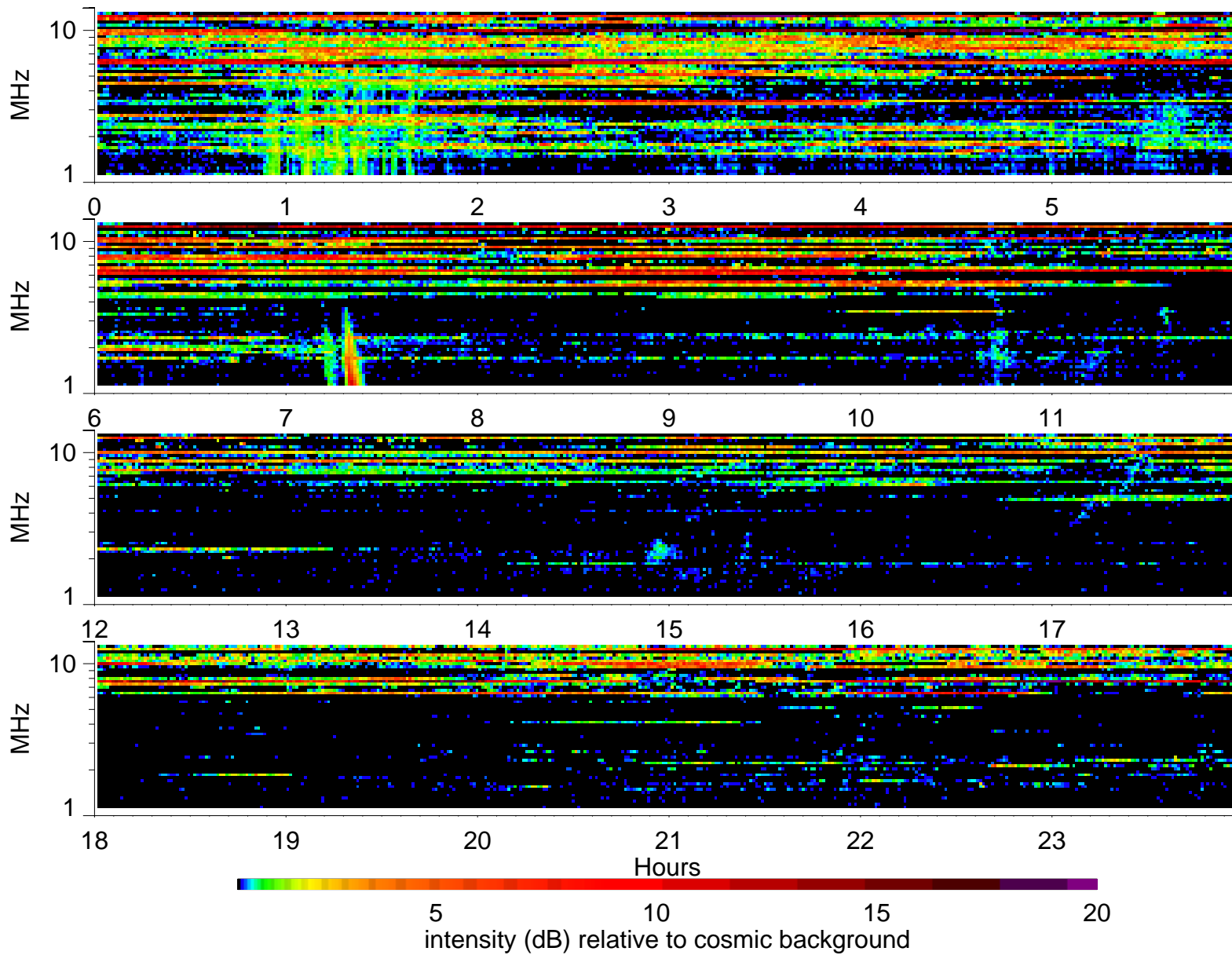
Wind Waves RAD2 receiver: 1996/4/20
