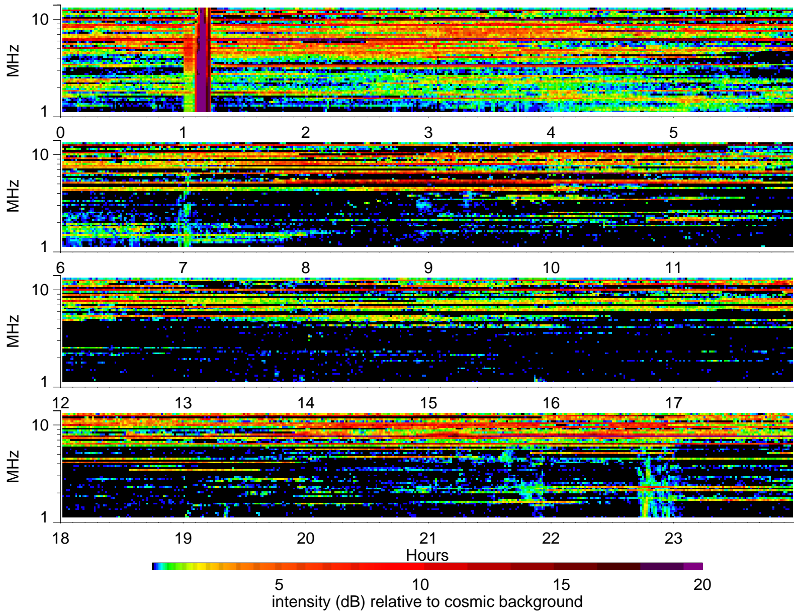
Wind Waves RAD2 receiver: 1996/4/19
