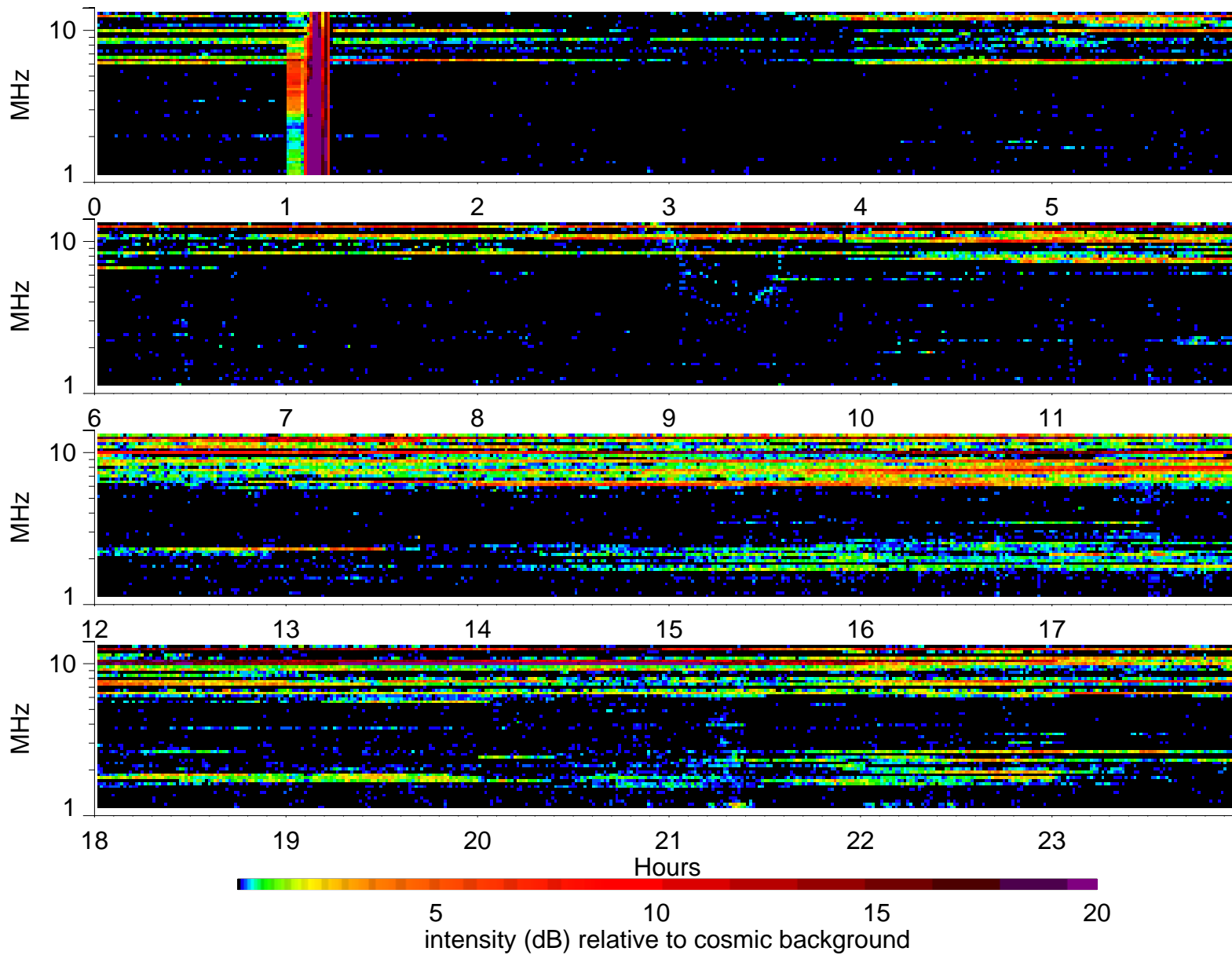
Wind Waves RAD2 receiver: 1996/4/15
