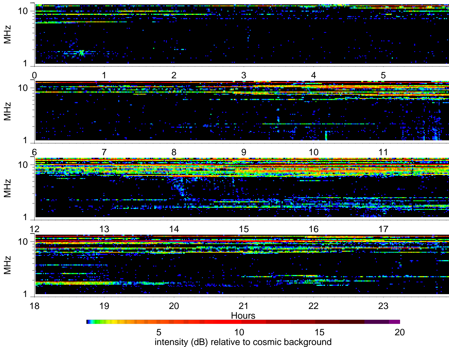
Wind Waves RAD2 receiver: 1996/4/14
