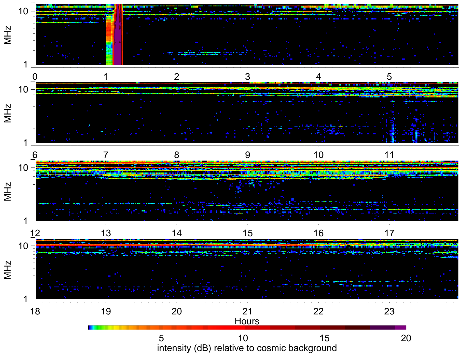
Wind Waves RAD2 receiver: 1996/4/13
