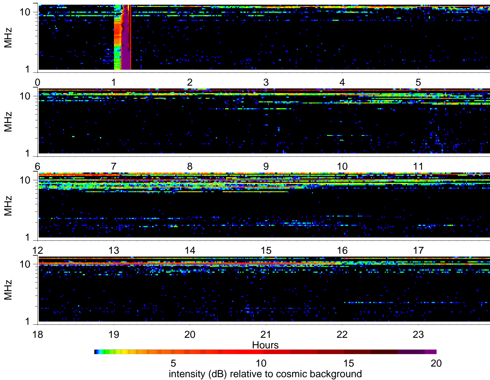
Wind Waves RAD2 receiver: 1996/4/11
