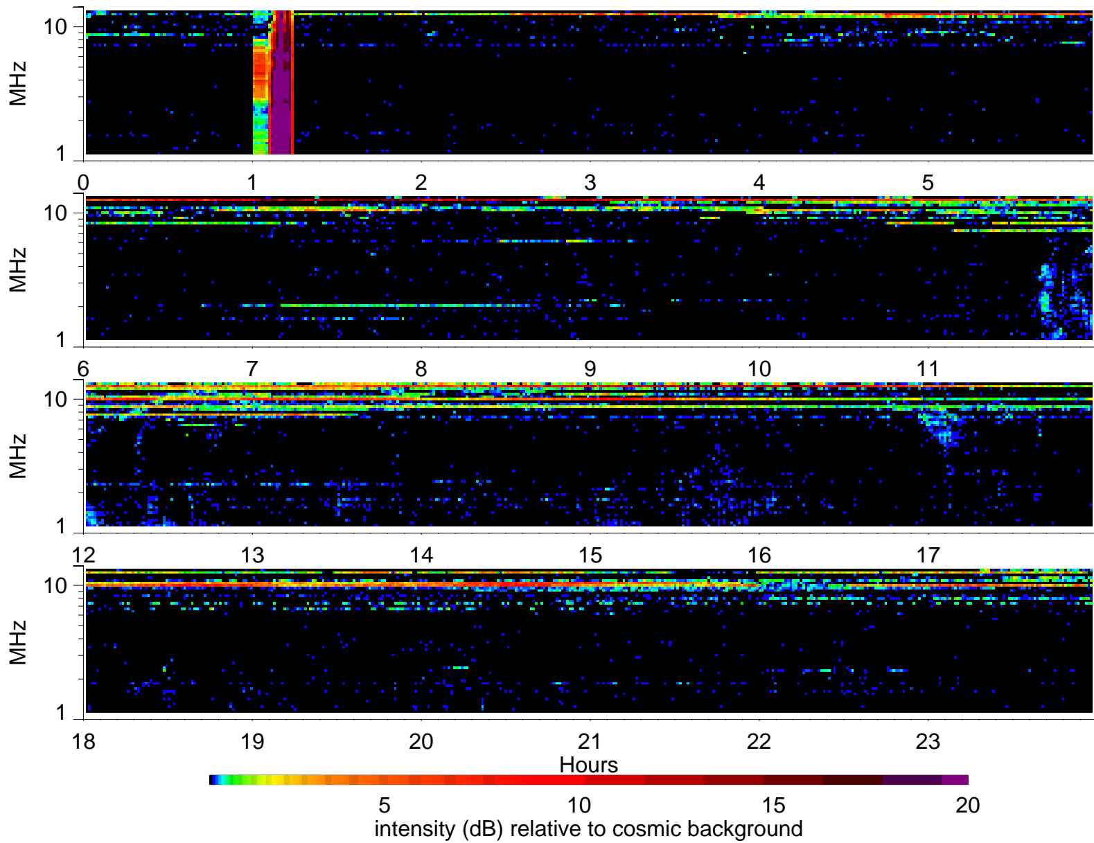
Wind Waves RAD2 receiver: 1996/4/9
