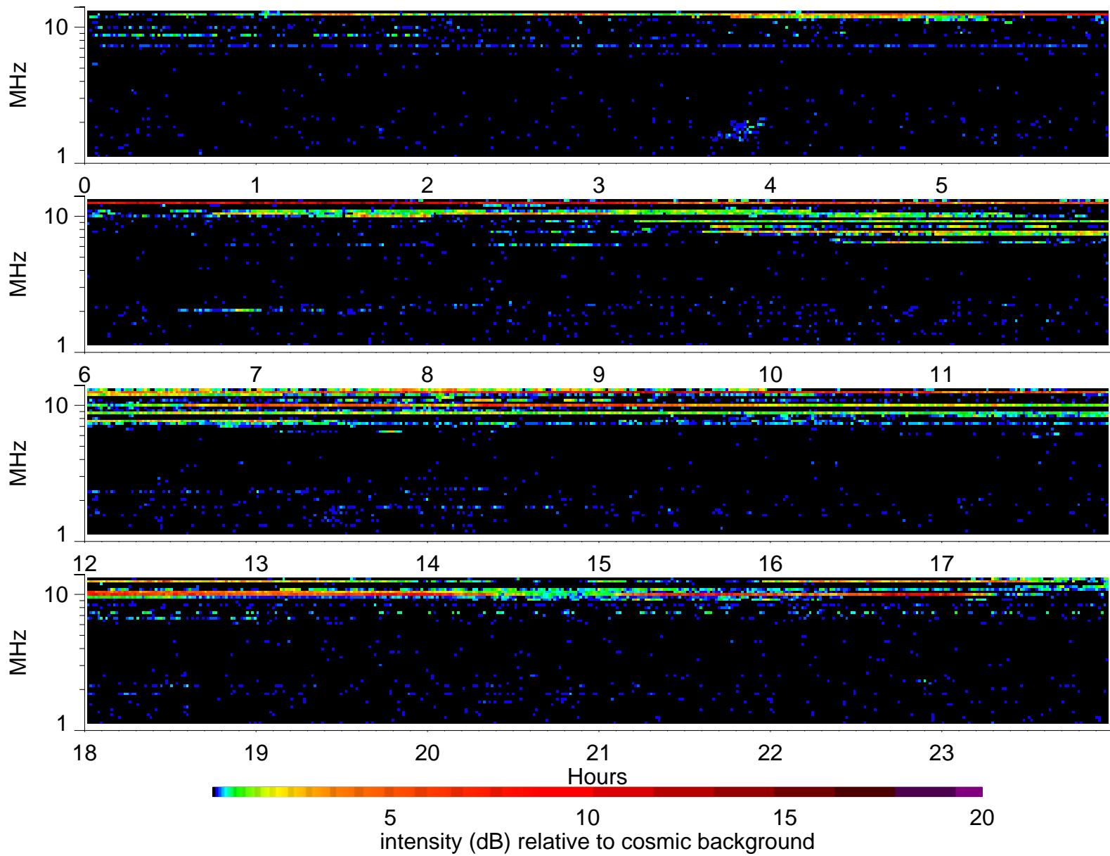
Wind Waves RAD2 receiver: 1996/4/6
