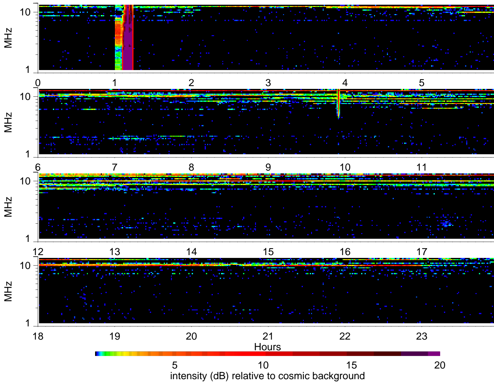
Wind Waves RAD2 receiver: 1996/4/5
