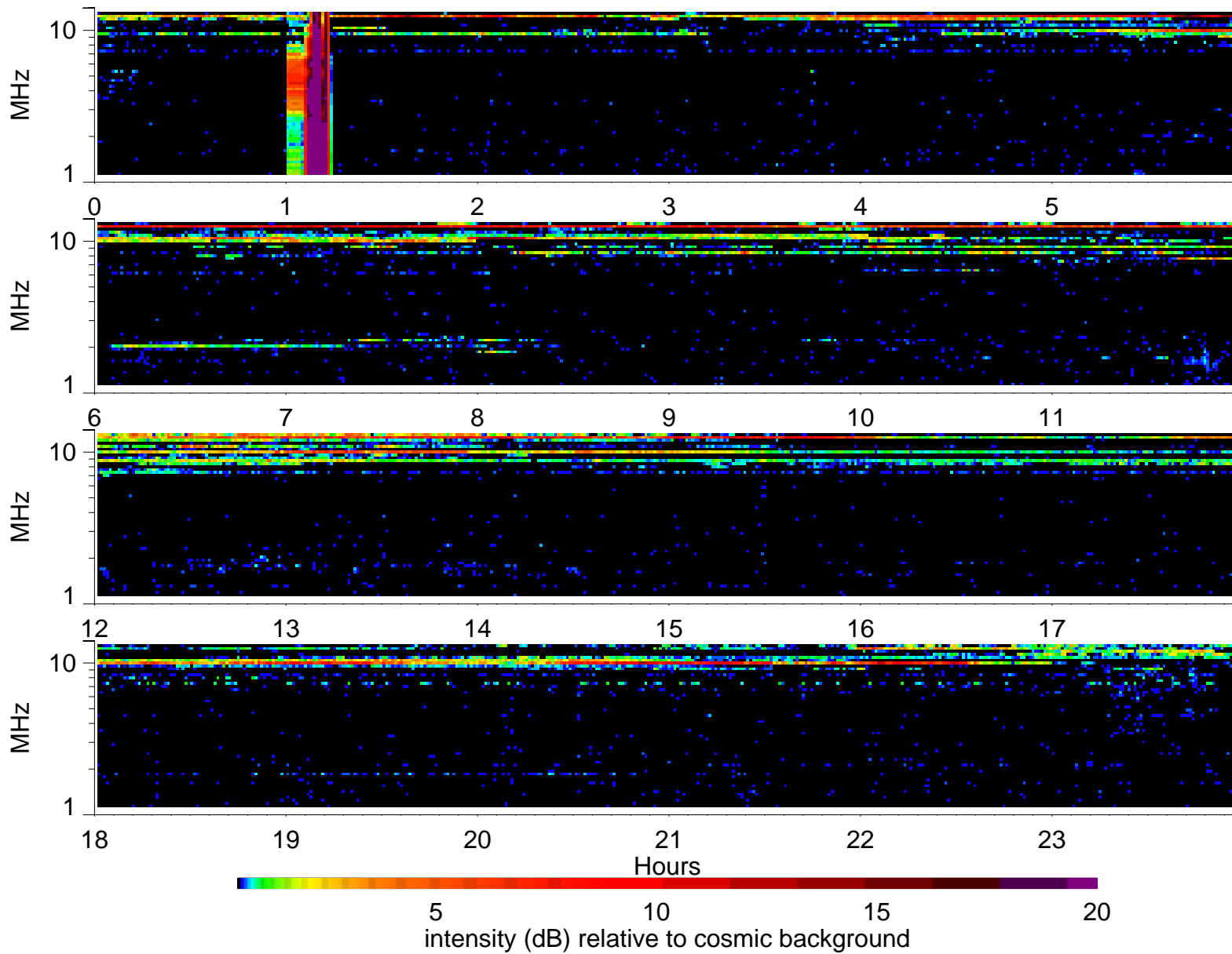
Wind Waves RAD2 receiver: 1996/4/3
