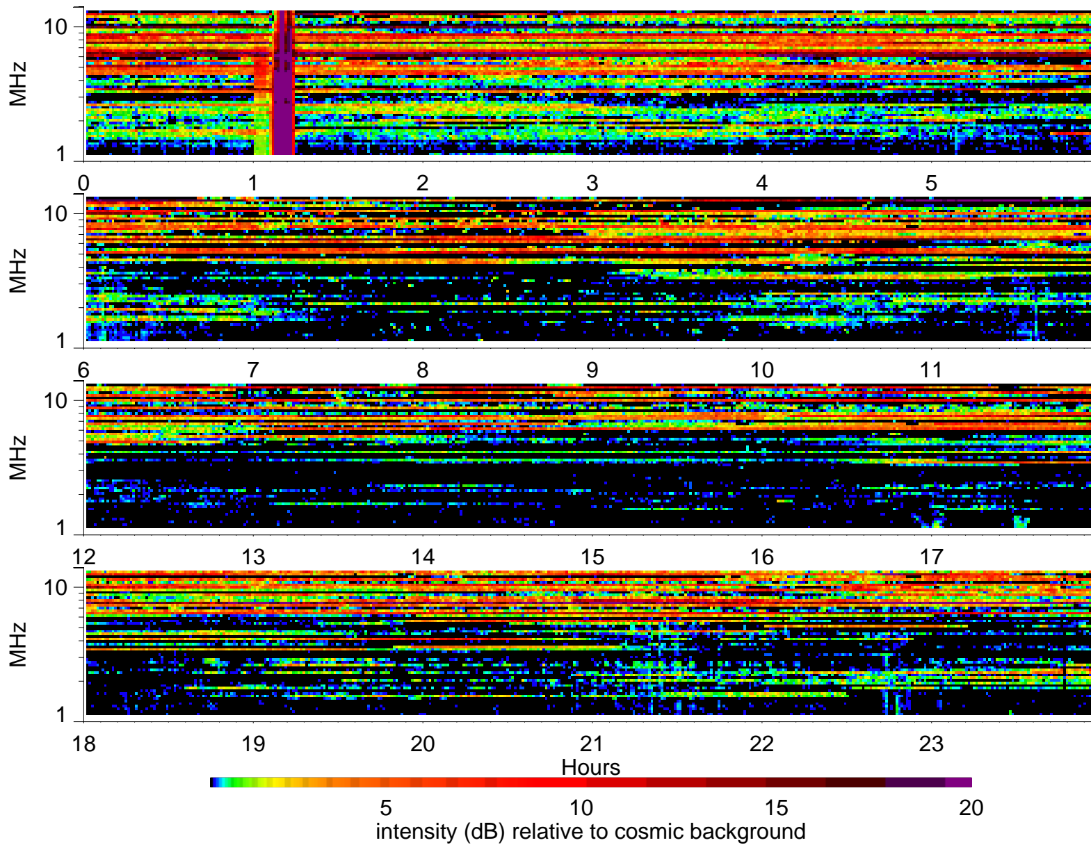
Wind Waves RAD2 receiver: 1996/3/28
