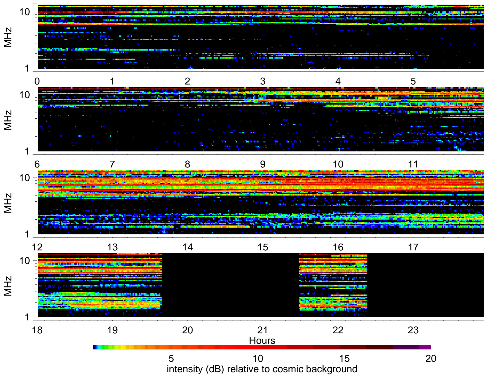
Wind Waves RAD2 receiver: 1996/3/25
